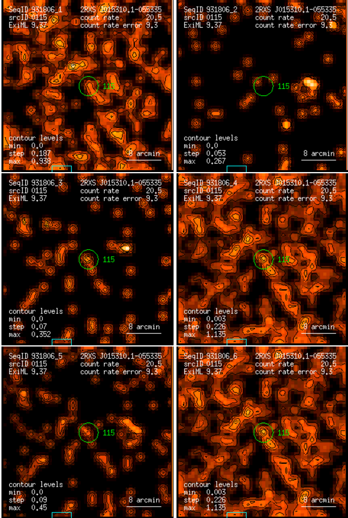
Figure 115: RASS 931806: detection 0115: band rate images, Gaussian filter: (1) PSPC channels 11 – 41, (2) 52 – 90, (3) 91 – 201, (4) 11 – 235, (5) 52 – 201, (6) 11 – 201. Broad band rates in counts/ks. Band rate contour levels in counts/ks/arcmin 2 .
