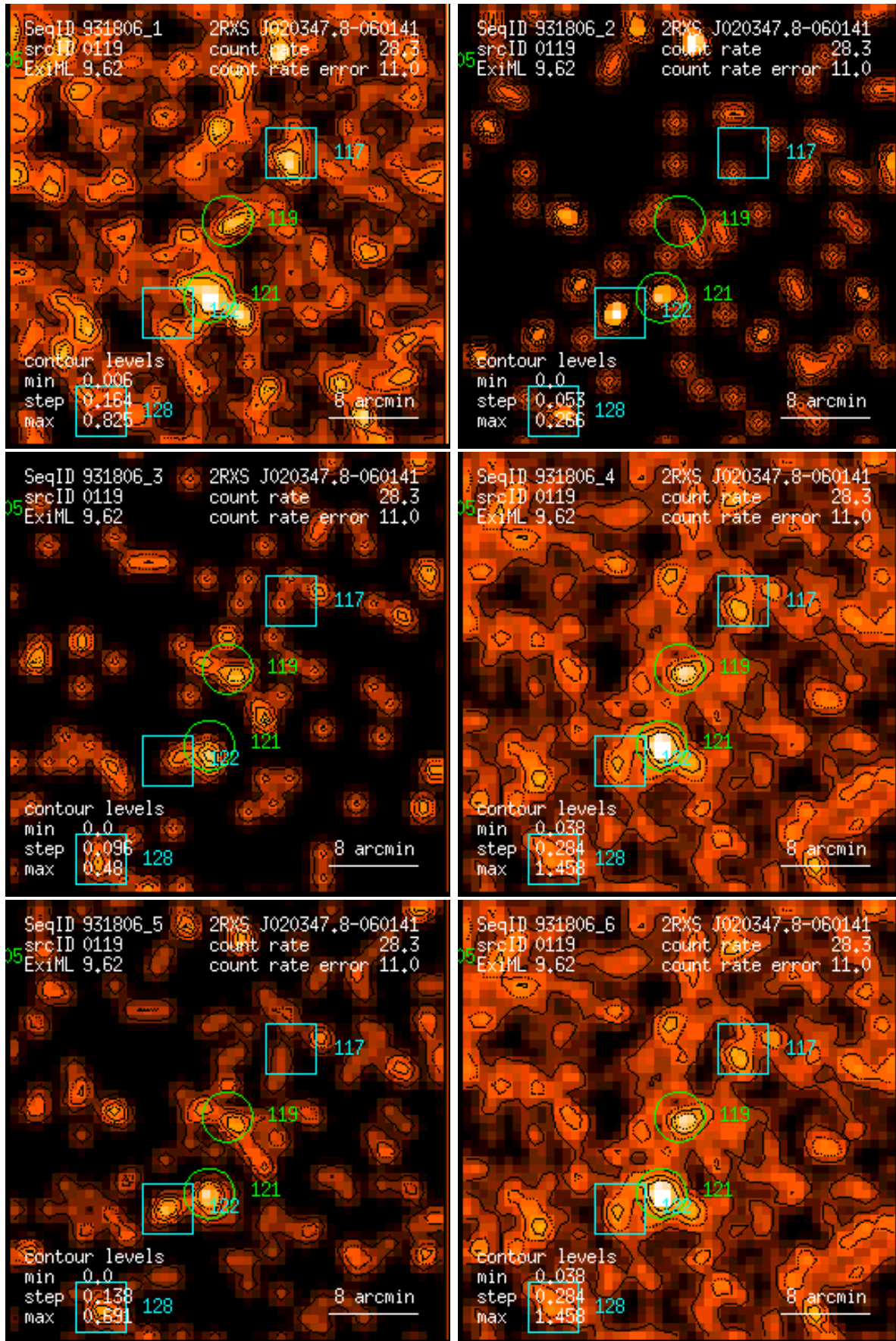
Figure 119: RASS 931806: detection 0119: band rate images, Gaussian filter: (1) PSPC channels 11 – 41, (2) 52 – 90, (3) 91 – 201, (4) 11 – 235, (5) 52 – 201, (6) 11 – 201. Broad band rates in counts/ks. Band rate contour levels in counts/ks/arcmin 2 .
