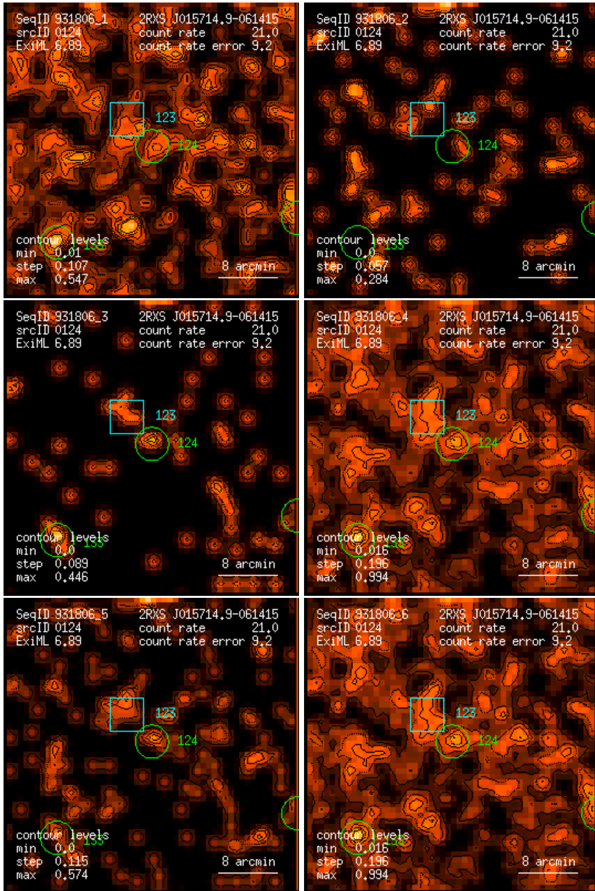
Figure 124: RASS 931806: detection 0124: band rate images, Gaussian filter: (1) PSPC channels 11 – 41, (2) 52 – 90, (3) 91 – 201, (4) 11 – 235, (5) 52 – 201, (6) 11 – 201. Broad band rates in counts/ks. Band rate contour levels in counts/ks/arcmin 2 .
