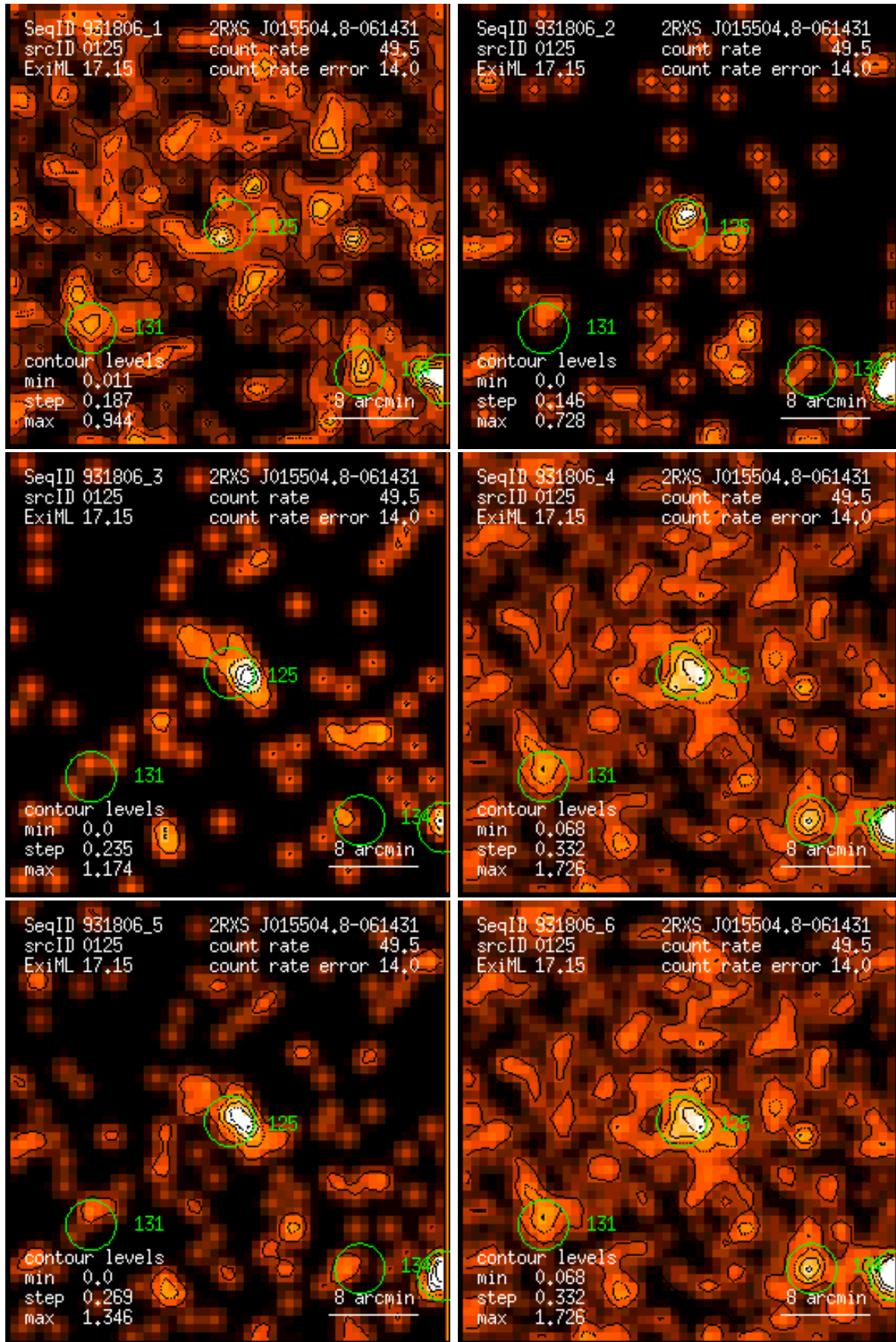
Figure 125: RASS 931806: detection 0125: band rate images, Gaussian filter: (1) PSPC channels 11 – 41, (2) 52 – 90, (3) 91 – 201, (4) 11 – 235, (5) 52 – 201, (6) 11 – 201. Broad band rates in counts/ks. Band rate contour levels in counts/ks/arcmin 2 .
