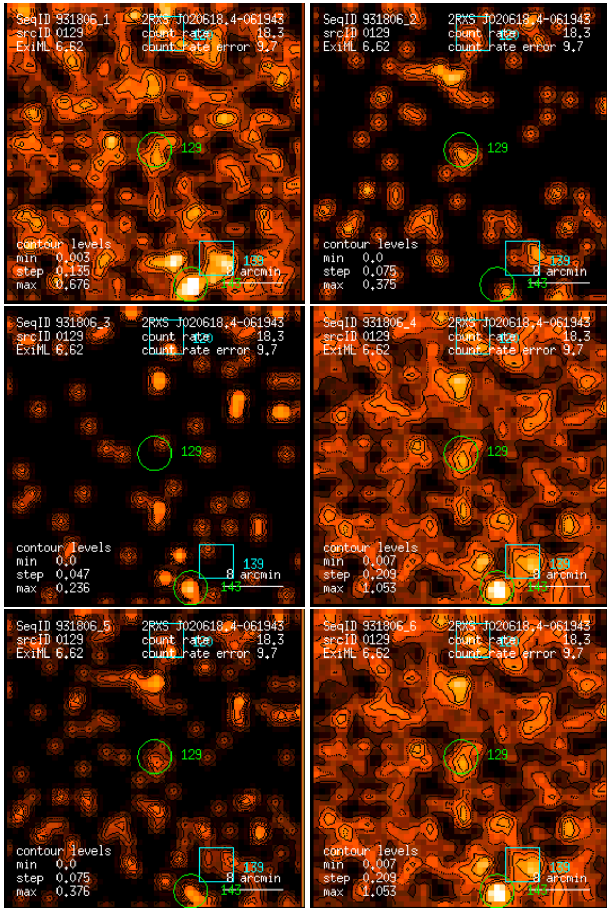
Figure 129: RASS 931806: detection 0129: band rate images, Gaussian filter: (1) PSPC channels 11 – 41, (2) 52 – 90, (3) 91 – 201, (4) 11 – 235, (5) 52 – 201, (6) 11 – 201. Broad band rates in counts/ks. Band rate contour levels in counts/ks/arcmin 2 .
