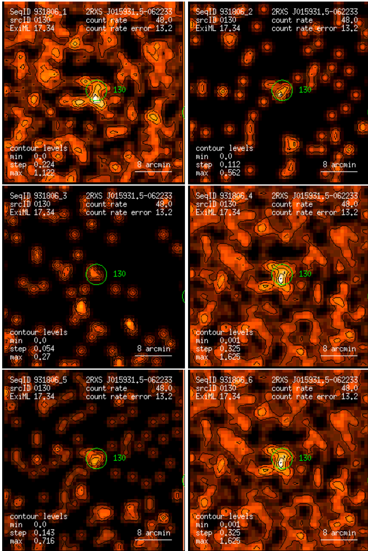
Figure 130: RASS 931806: detection 0130: band rate images, Gaussian filter: (1) PSPC channels 11 – 41, (2) 52 – 90, (3) 91 – 201, (4) 11 – 235, (5) 52 – 201, (6) 11 – 201. Broad band rates in counts/ks. Band rate contour levels in counts/ks/arcmin 2 .
