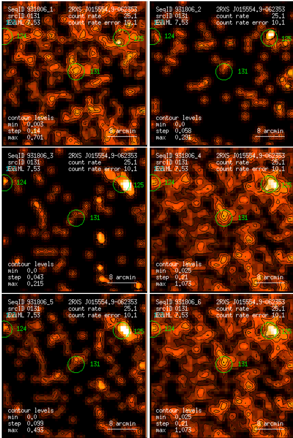
Figure 131: RASS 931806: detection 0131: band rate images, Gaussian filter: (1) PSPC channels 11 – 41, (2) 52 – 90, (3) 91 – 201, (4) 11 – 235, (5) 52 – 201, (6) 11 – 201. Broad band rates in counts/ks. Band rate contour levels in counts/ks/arcmin 2 .
