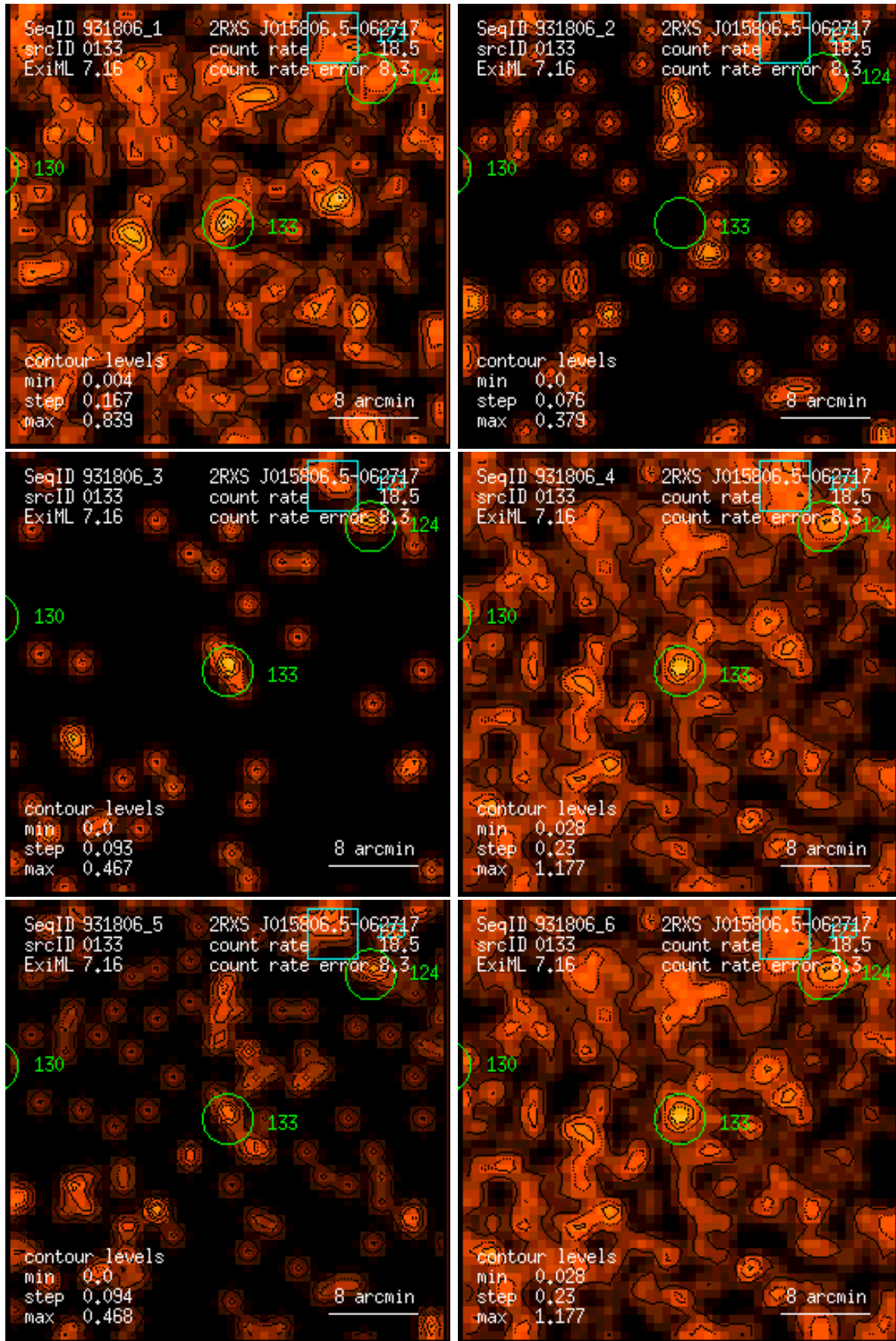
Figure 133: RASS 931806: detection 0133: band rate images, Gaussian filter: (1) PSPC channels 11 – 41, (2) 52 – 90, (3) 91 – 201, (4) 11 – 235, (5) 52 – 201, (6) 11 – 201. Broad band rates in counts/ks. Band rate contour levels in counts/ks/arcmin 2 .
