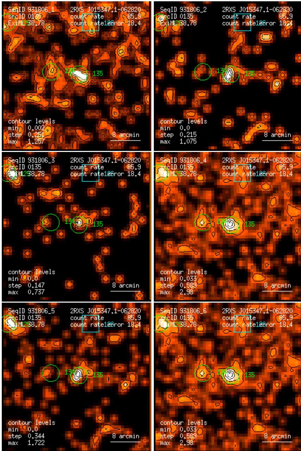
Figure 135: RASS 931806: detection 0135: band rate images, Gaussian filter: (1) PSPC channels 11 – 41, (2) 52 – 90, (3) 91 – 201, (4) 11 – 235, (5) 52 – 201, (6) 11 – 201. Broad band rates in counts/ks. Band rate contour levels in counts/ks/arcmin 2 .
