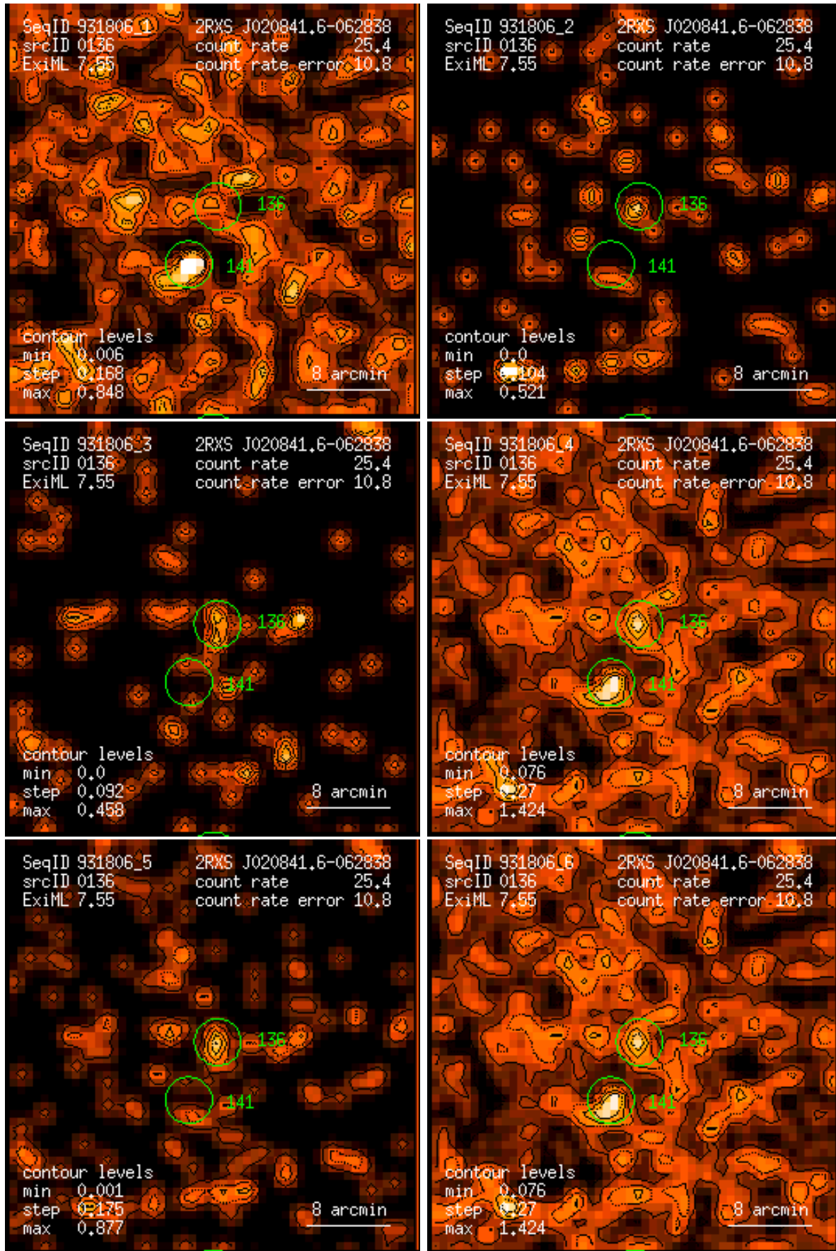
Figure 136: RASS 931806: detection 0136: band rate images, Gaussian filter: (1) PSPC channels 11 – 41, (2) 52 – 90, (3) 91 – 201, (4) 11 – 235, (5) 52 – 201, (6) 11 – 201. Broad band rates in counts/ks. Band rate contour levels in counts/ks/arcmin 2 .
