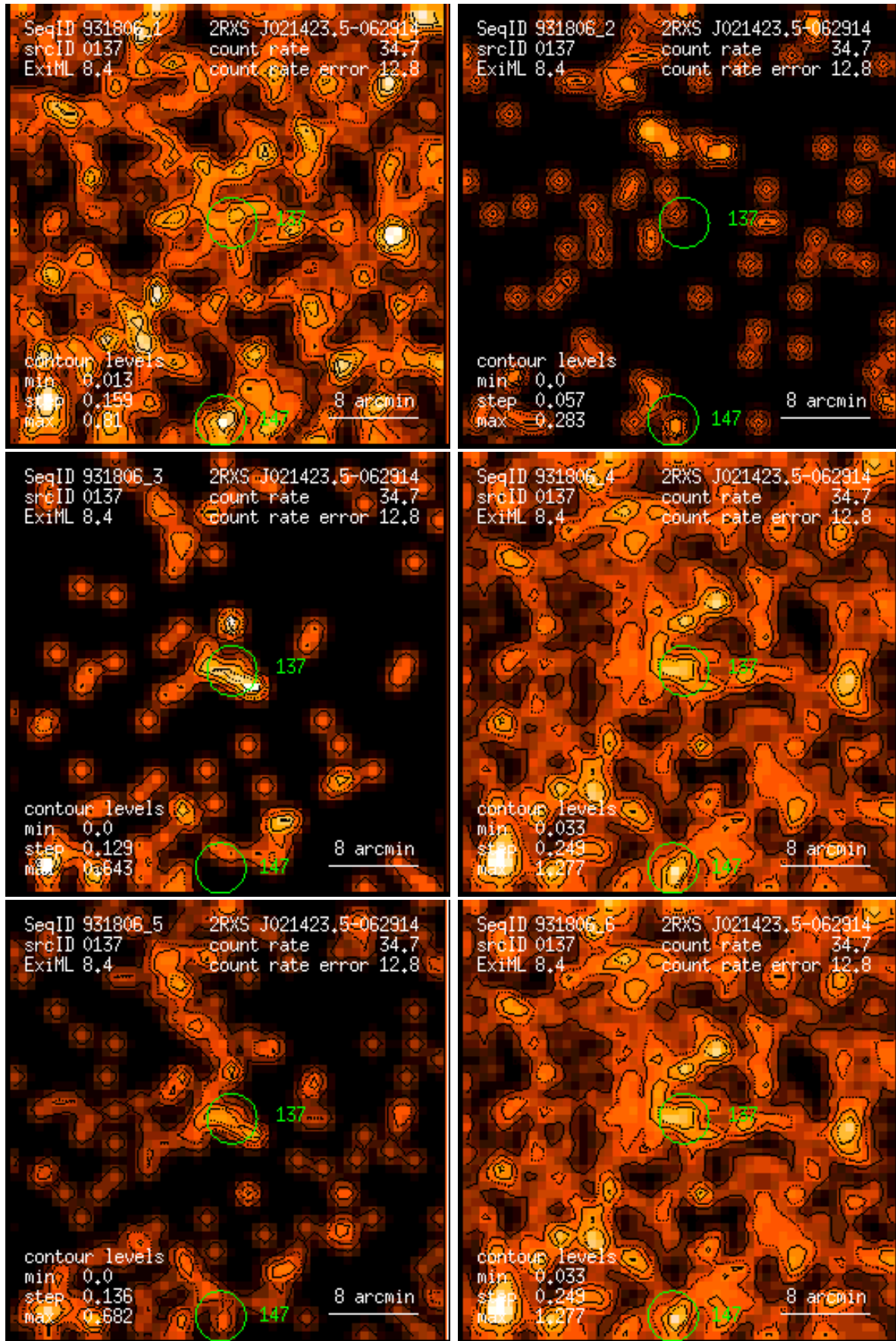
Figure 137: RASS 931806: detection 0137: band rate images, Gaussian filter: (1) PSPC channels 11 – 41, (2) 52 – 90, (3) 91 – 201, (4) 11 – 235, (5) 52 – 201, (6) 11 – 201. Broad band rates in counts/ks. Band rate contour levels in counts/ks/arcmin 2 .
