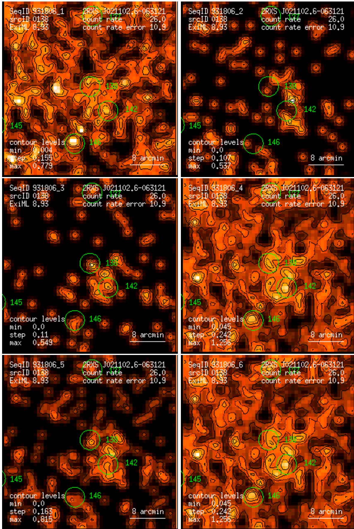
Figure 138: RASS 931806: detection 0138: band rate images, Gaussian filter: (1) PSPC channels 11 – 41, (2) 52 – 90, (3) 91 – 201, (4) 11 – 235, (5) 52 – 201, (6) 11 – 201. Broad band rates in counts/ks. Band rate contour levels in counts/ks/arcmin 2 .
