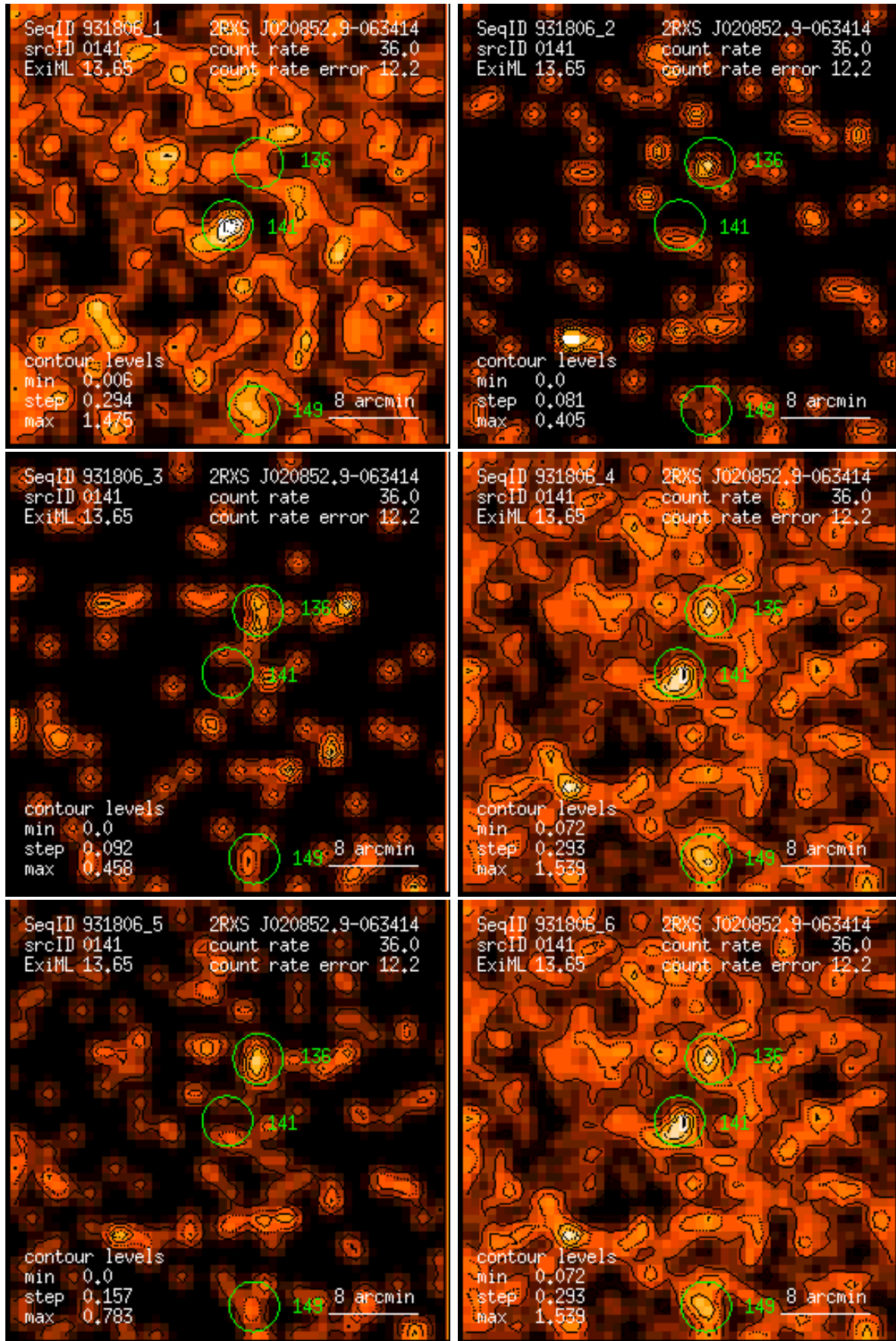
Figure 141: RASS 931806: detection 0141: band rate images, Gaussian filter: (1) PSPC channels 11 – 41, (2) 52 – 90, (3) 91 – 201, (4) 11 – 235, (5) 52 – 201, (6) 11 – 201. Broad band rates in counts/ks. Band rate contour levels in counts/ks/arcmin 2 .
