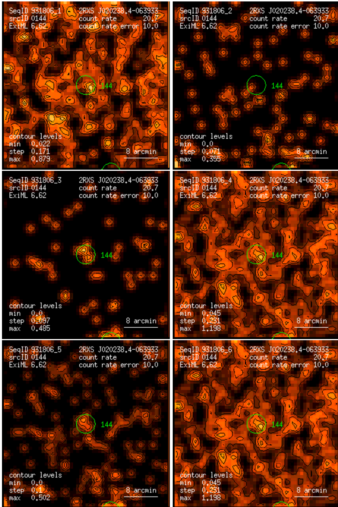
Figure 144: RASS 931806: detection 0144: band rate images, Gaussian filter: (1) PSPPC channels 11 – 41, (2) 52 – 90, (3) 91 – 201, (4) 11 – 235, (5) 52 – 201, (6) 11 – 201. Broad band rates in counts/ks. Band rate contour levels in counts/ks/arcmin 2 .
