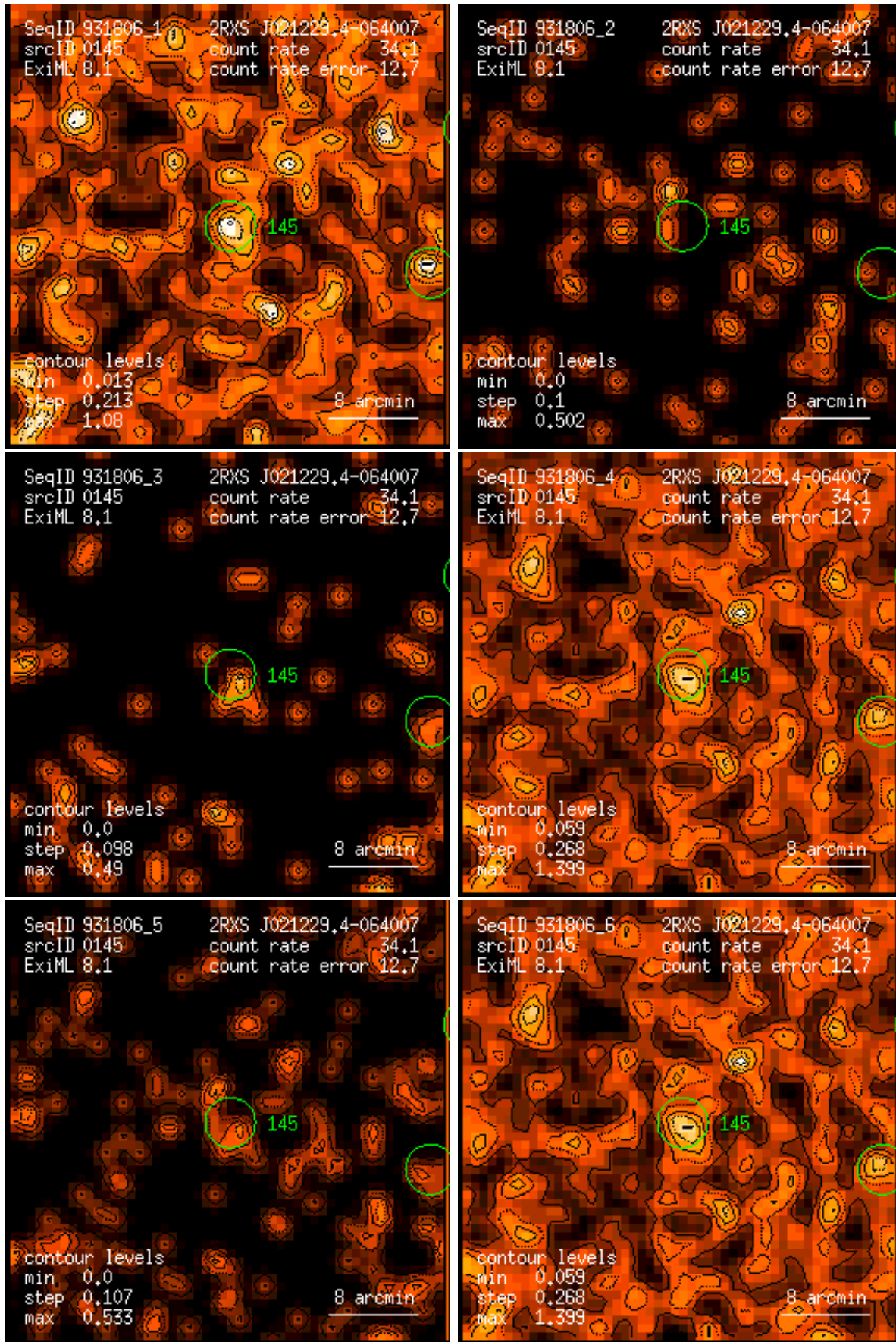
Figure 145: RASS 931806: detection 0145: band rate images, Gaussian filter: (1) PSPC channels 11 – 41, (2) 52 – 90, (3) 91 – 201, (4) 11 – 235, (5) 52 – 201, (6) 11 – 201. Broad band rates in counts/ks. Band rate contour levels in counts/ks/arcmin 2 .
