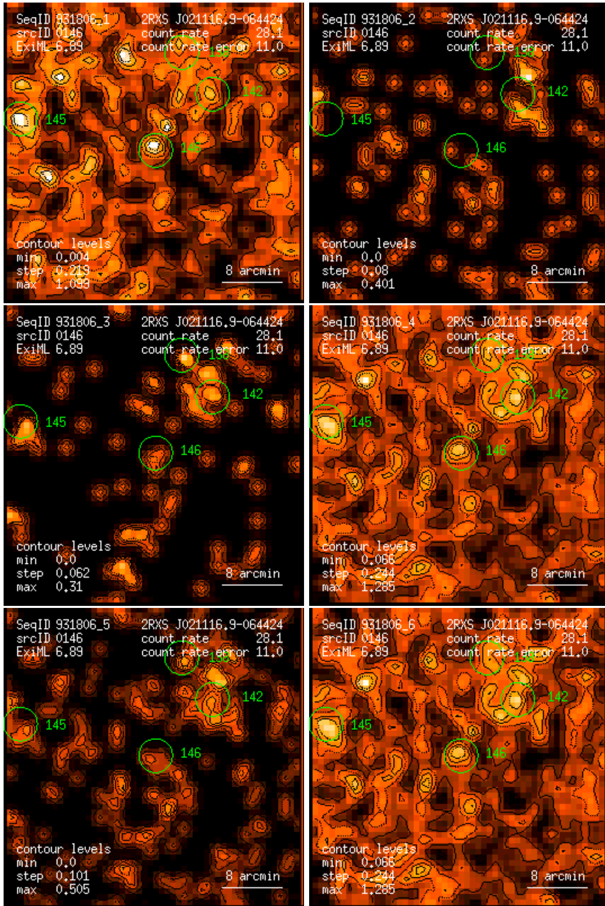
Figure 146: RASS 931806: detection 0146: band rate images, Gaussian filter: (1) PSPC channels 11 – 41, (2) 52 – 90, (3) 91 – 201, (4) 11 – 235, (5) 52 – 201, (6) 11 – 201. Broad band rates in counts/ks. Band rate contour levels in counts/ks/arcmin 2 .
