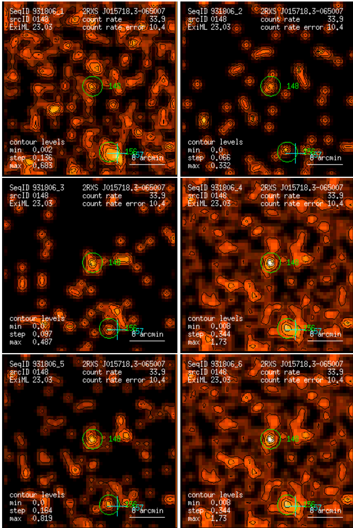
Figure 148: RASS 931806: detection 0148: band rate images, Gaussian filter: (1) PSPC channels 11 – 41, (2) 52 – 90, (3) 91 – 201, (4) 11 – 235, (5) 52 – 201, (6) 11 – 201. Broad band rates in counts/ks. Band rate contour levels in counts/ks/arcmin 2 .
