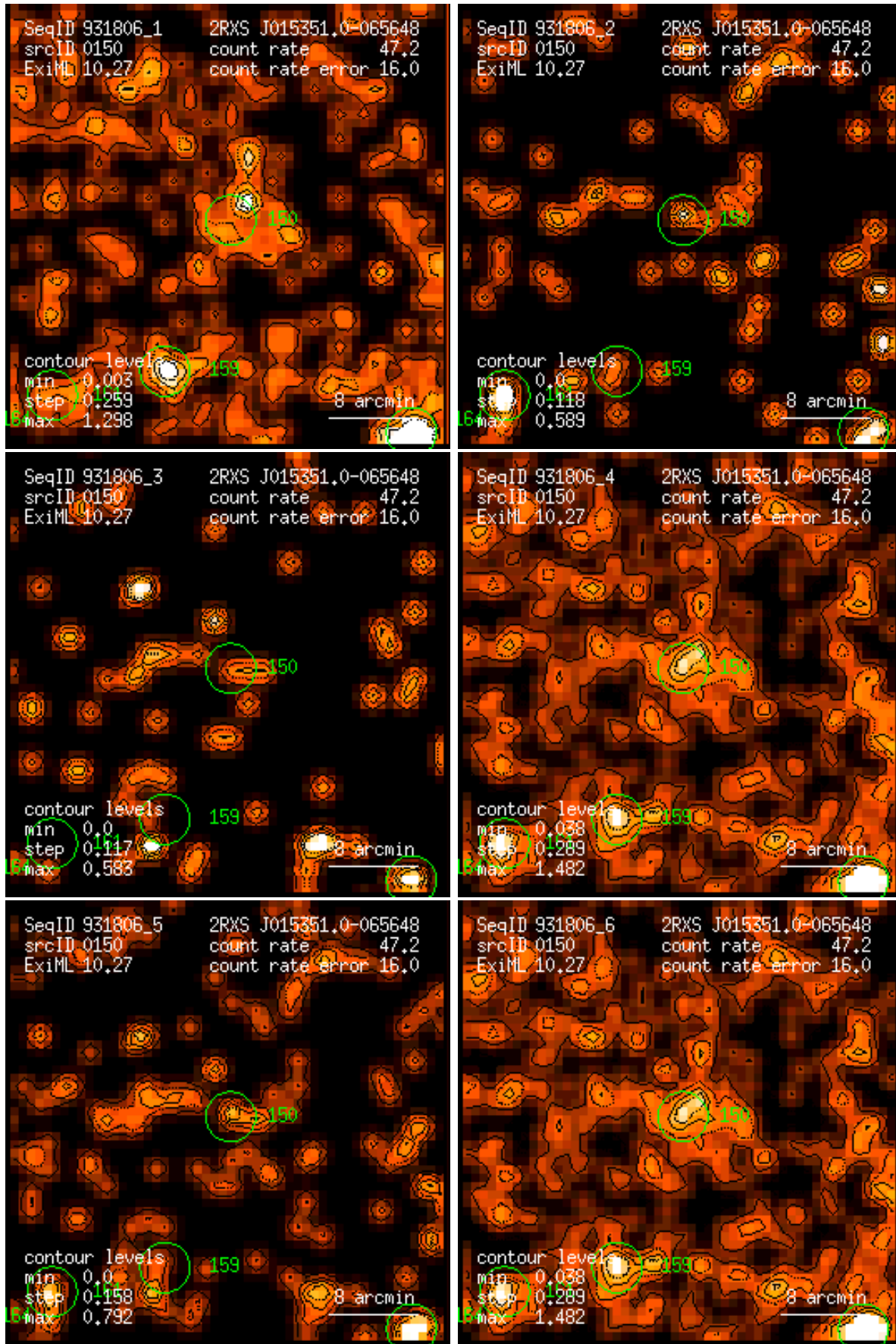
Figure 150: RASS 931806: detection 0150: band rate images, Gaussian filter: (1) PSPC channels 11 – 41, (2) 52 – 90, (3) 91 – 201, (4) 11 – 235, (5) 52 – 201, (6) 11 – 201. Broad band rates in counts/ks. Band rate contour levels in counts/ks/arcmin 2 .
