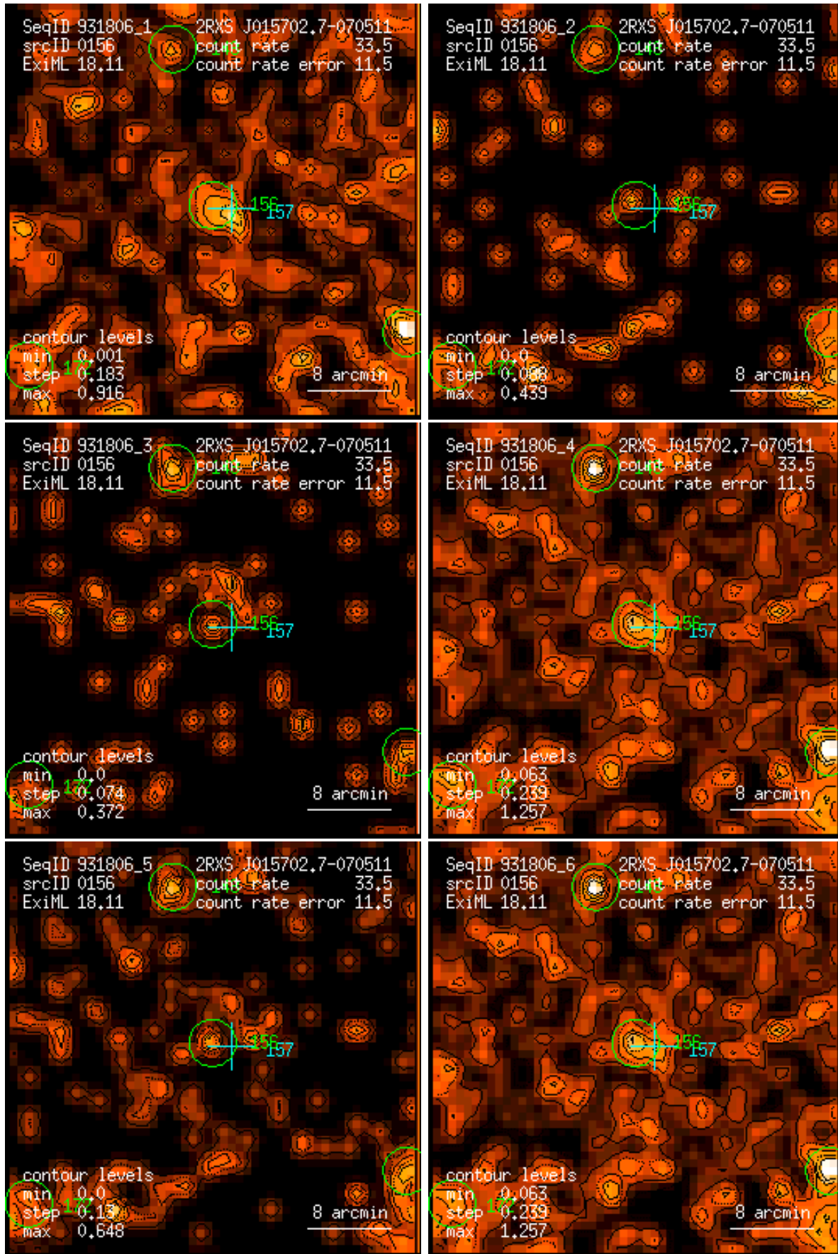
Figure 156: RASS 931806: detection 0156: band rate images, Gaussian filter: (1) PSPC channels 11 – 41, (2) 52 – 90, (3) 91 – 201, (4) 11 – 235, (5) 52 – 201, (6) 11 – 201. Broad band rates in counts/ks. Band rate contour levels in counts/ks/arcmin 2 .
