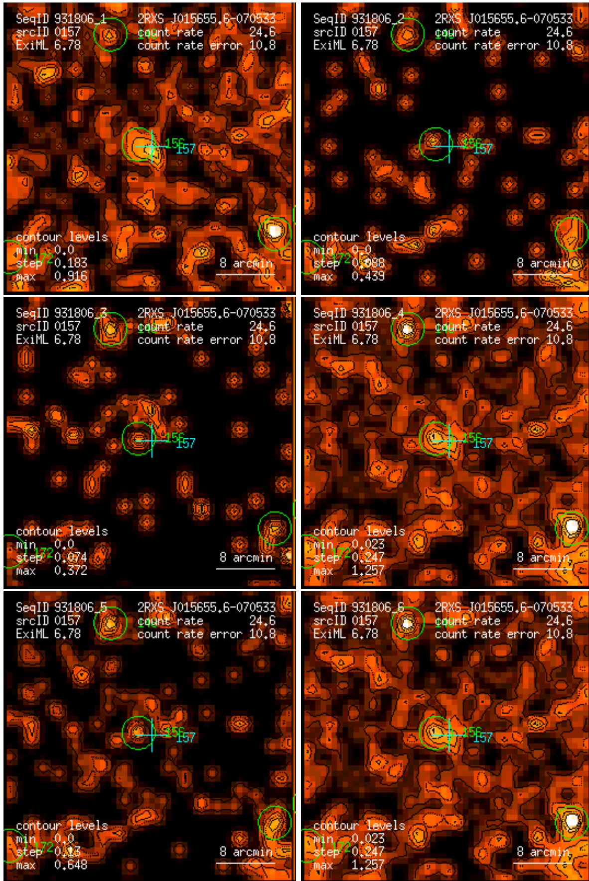
Figure 157: RASS 931806: detection 0157: band rate images, Gaussian filter: (1) PSPC channels 11 – 41, (2) 52 – 90, (3) 91 – 201, (4) 11 – 235, (5) 52 – 201, (6) 11 – 201. Broad band rates in counts/ks. Band rate contour levels in counts/ks/arcmin 2 .
