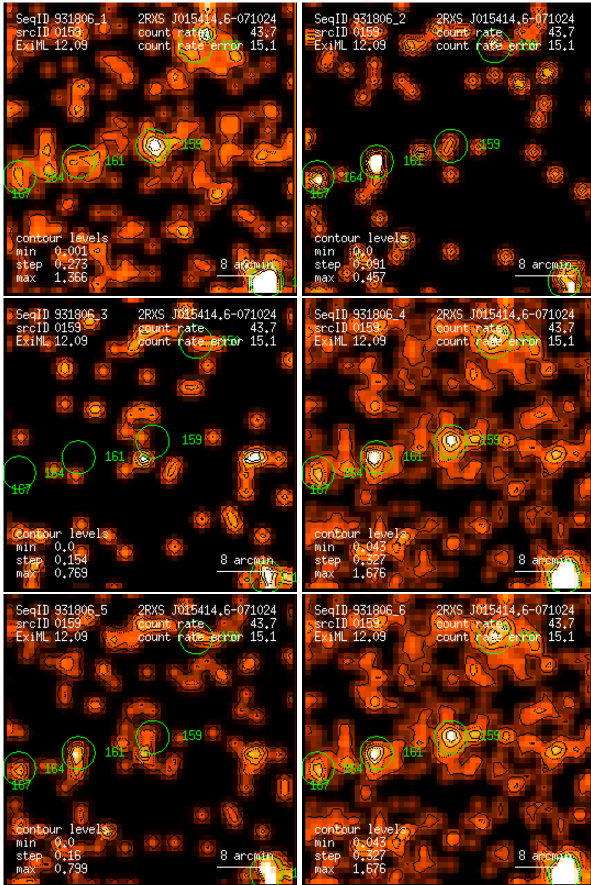
Figure 159: RASS 931806: detection 0159: band rate images, Gaussian filter: (1) PSPC channels 11 – 41, (2) 52 – 90, (3) 91 – 201, (4) 11 – 235, (5) 52 – 201, (6) 11 – 201. Broad band rates in counts/ks. Band rate contour levels in counts/ks/arcmin 2 .
