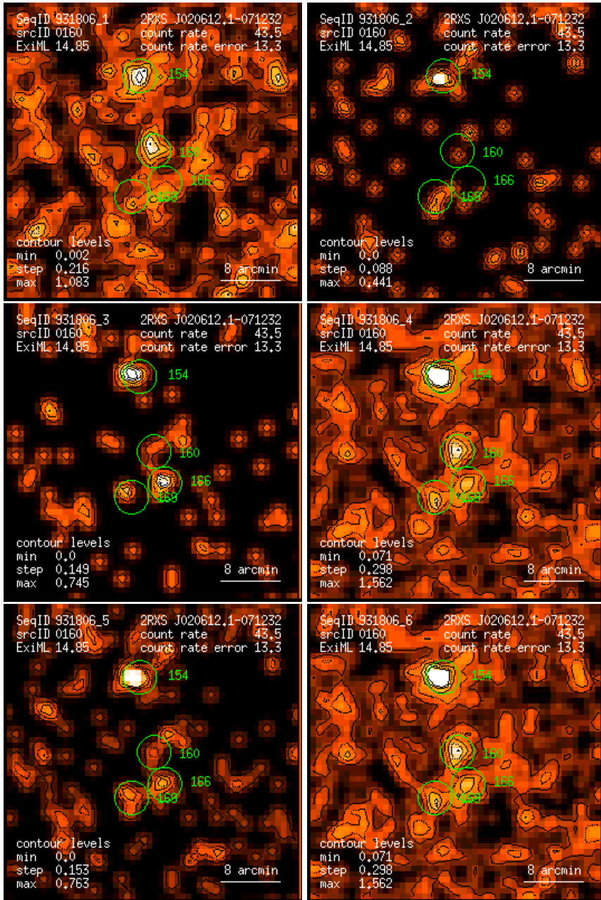
Figure 160: RASS 931806: detection 0160: band rate images, Gaussian filter: (1) PSPC channels 11 – 41, (2) 52 – 90, (3) 91 – 201, (4) 11 – 235, (5) 52 – 201, (6) 11 – 201. Broad band rates in counts/ks. Band rate contour levels in counts/ks/arcmin 2 .
