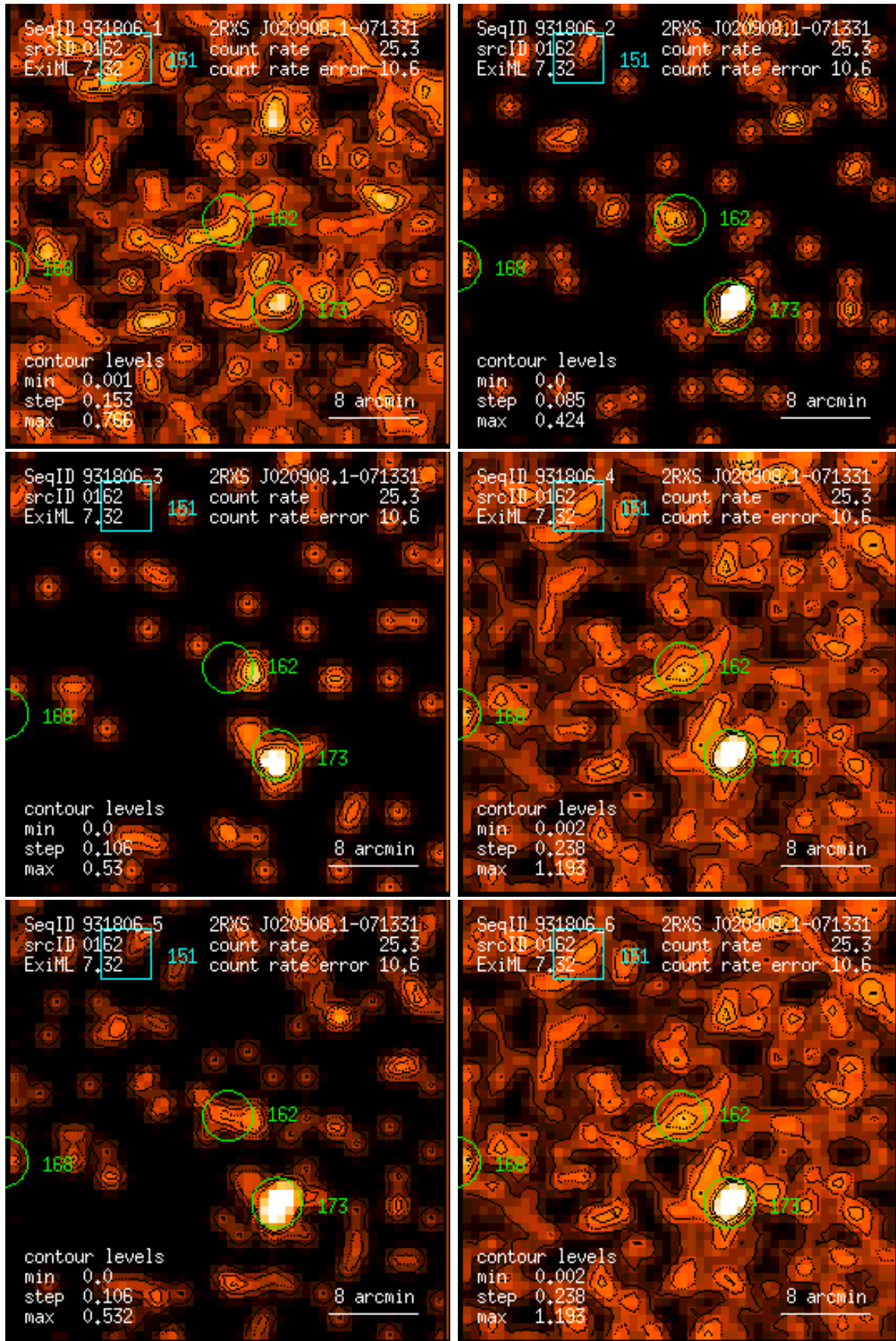
Figure 162: RASS 931806: detection 0162: band rate images, Gaussian filter: (1) PSPC channels 11 – 41, (2) 52 – 90, (3) 91 – 201, (4) 11 – 235, (5) 52 – 201, (6) 11 – 201. Broad band rates in counts/ks. Band rate contour levels in counts/ks/arcmin 2 .
