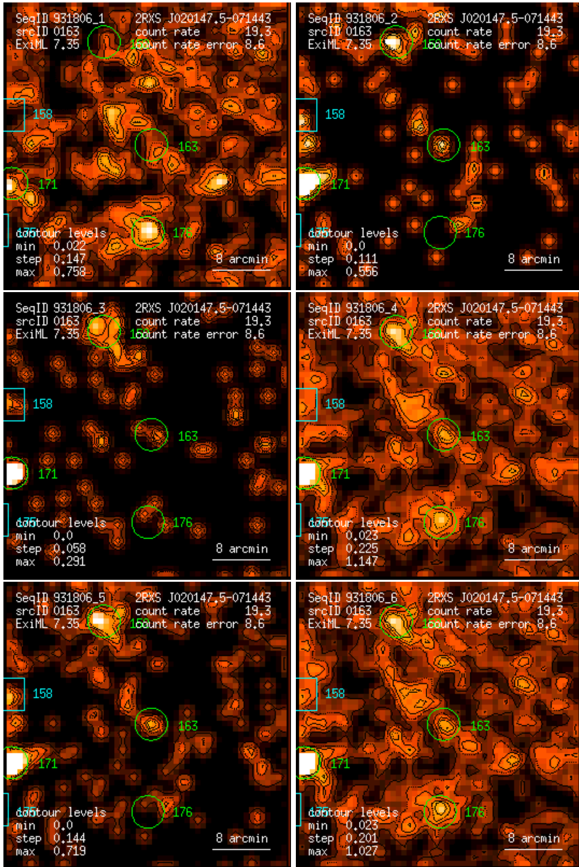
Figure 163: RASS 931806: detection 0163: band rate images, Gaussian filter: (1) PSPC channels 11 – 41, (2) 52 – 90, (3) 91 – 201, (4) 11 – 235, (5) 52 – 201, (6) 11 – 201. Broad band rates in counts/ks. Band rate contour levels in counts/ks/arcmin 2 .
