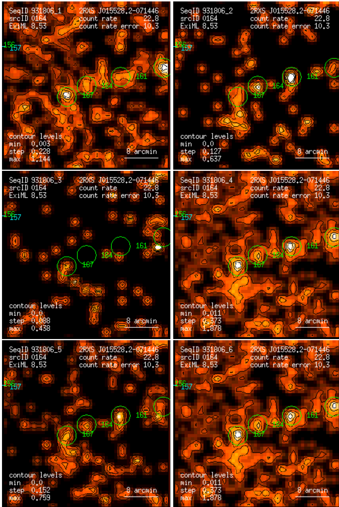
Figure 164: RASS 931806: detection 0164: band rate images, Gaussian filter: (1) PSPC channels 11 – 41, (2) 52 – 90, (3) 91 – 201, (4) 11 – 235, (5) 52 – 201, (6) 11 – 201. Broad band rates in counts/ks. Band rate contour levels in counts/ks/arcmin 2 .
