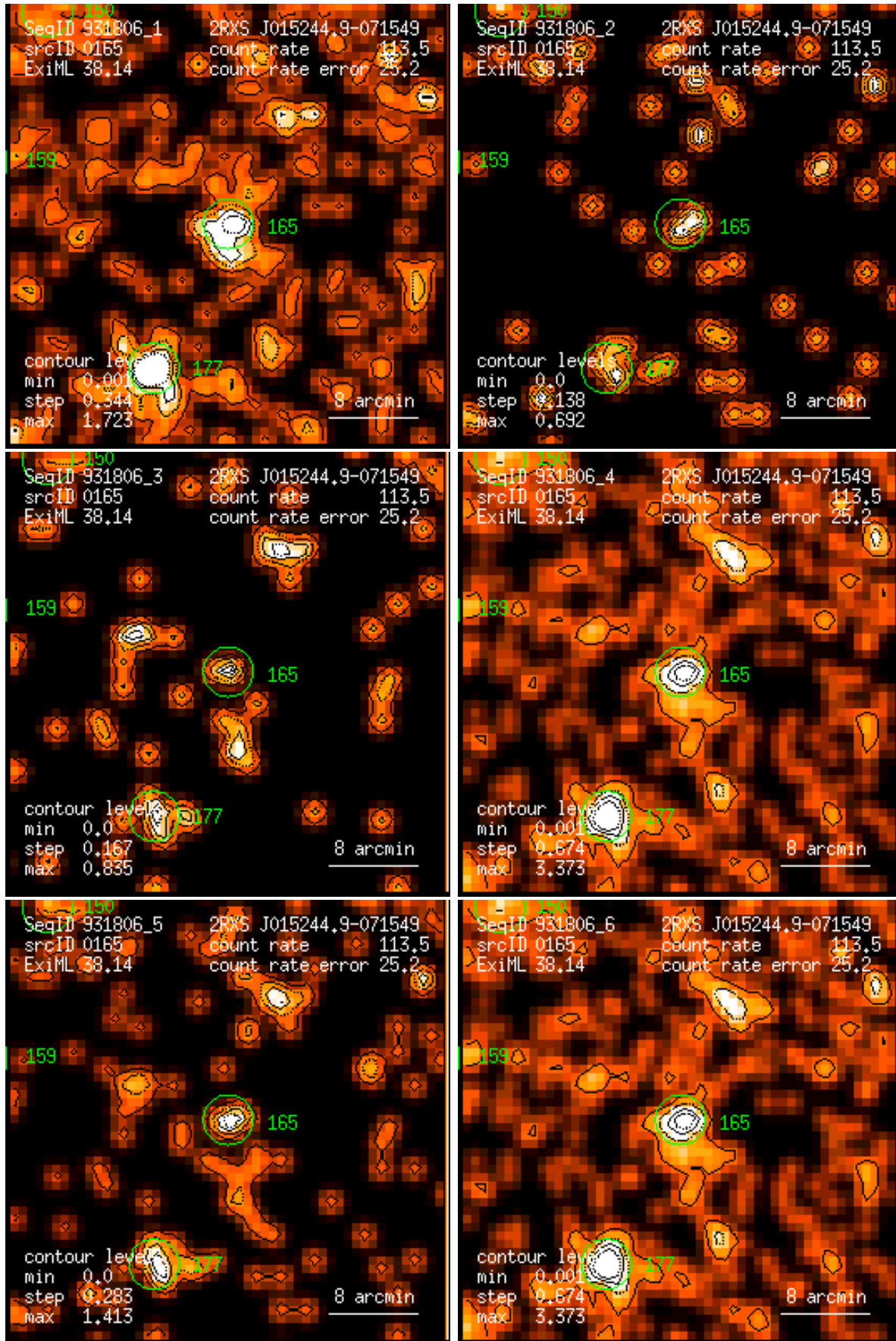
Figure 165: RASS 931806: detection 0165: band rate images, Gaussian filter: (1) PSPC channels 11 – 41, (2) 52 – 90, (3) 91 – 201, (4) 11 – 235, (5) 52 – 201, (6) 11 – 201. Broad band rates in counts/ks. Band rate contour levels in counts/ks/arcmin 2 .
