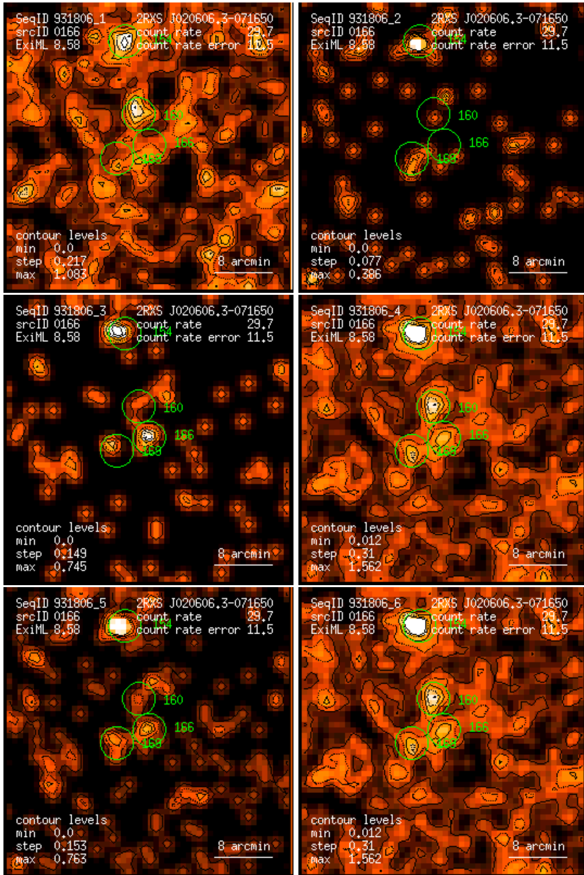
Figure 166: RASS 931806: detection 0166: band rate images, Gaussian filter: (1) PSPC channels 11 – 41, (2) 52 – 90, (3) 91 – 201, (4) 11 – 235, (5) 52 – 201, (6) 11 – 201. Broad band rates in counts/ks. Band rate contour levels in counts/ks/arcmin 2 .
