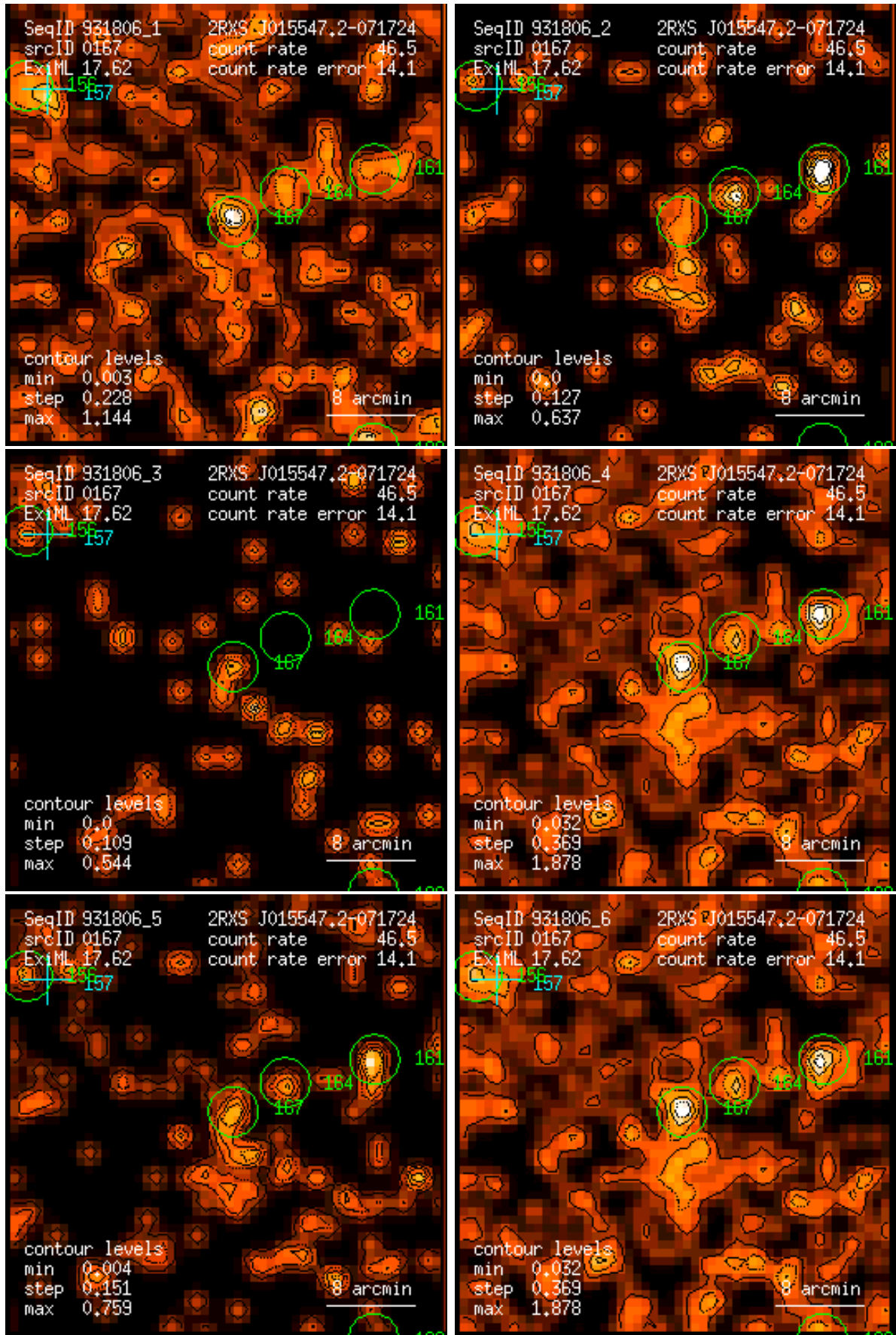
Figure 167: RASS 931806: detection 0167: band rate images, Gaussian filter: (1) PSPC channels 11 – 41, (2) 52 – 90, (3) 91 – 201, (4) 11 – 235, (5) 52 – 201, (6) 11 – 201. Broad band rates in counts/ks. Band rate contour levels in counts/ks/arcmin 2 .
