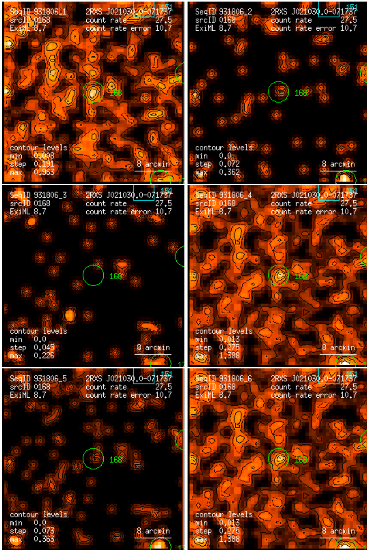
Figure 168: RASS 931806: detection 0168: band rate images, Gaussian filter: (1) PSPC channels 11 – 41, (2) 52 – 90, (3) 91 – 201, (4) 11 – 235, (5) 52 – 201, (6) 11 – 201. Broad band rates in counts/ks. Band rate contour levels in counts/ks/arcmin 2 .
