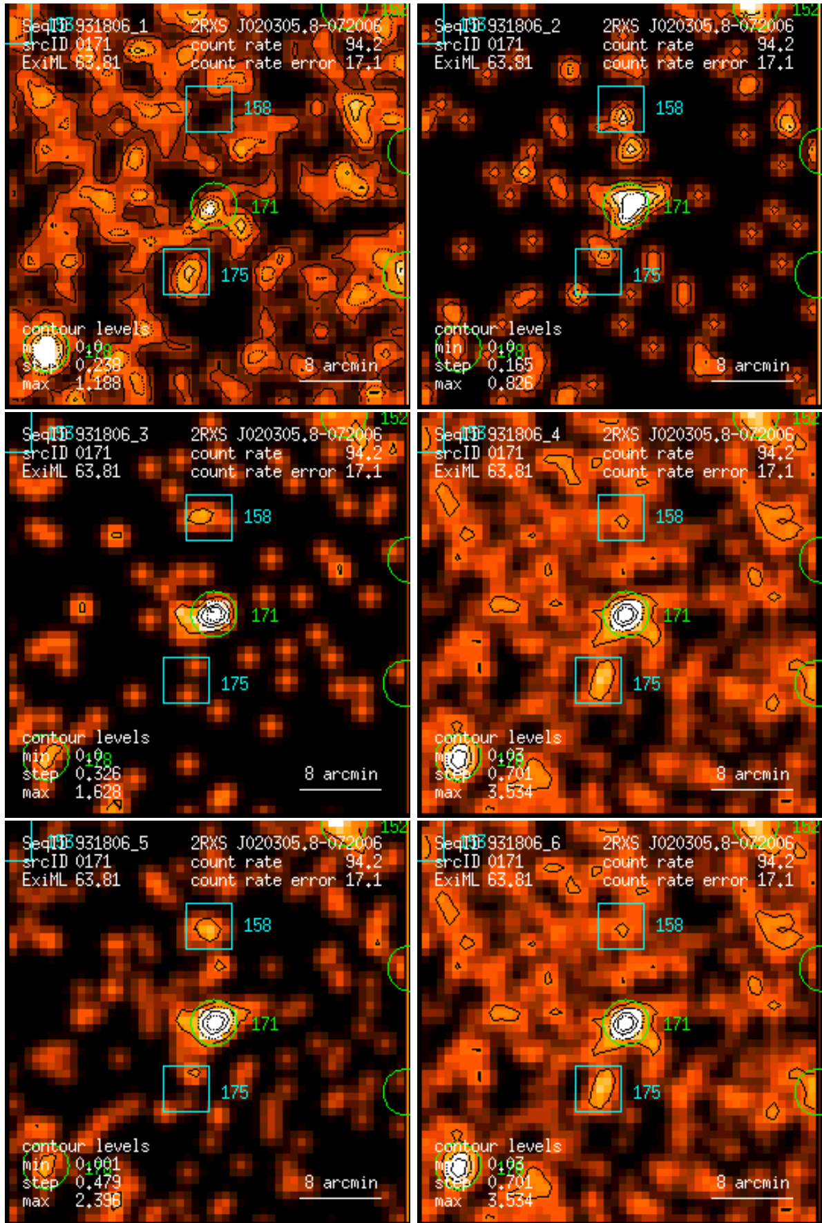
Figure 171: RASS 931806: detection 0171: band rate images, Gaussian filter: (1) PSPC channels 11 – 41, (2) 52 – 90, (3) 91 – 201, (4) 11 – 235, (5) 52 – 201, (6) 11 – 201. Broad band rates in counts/ks. Band rate contour levels in counts/ks/arcmin 2 .
