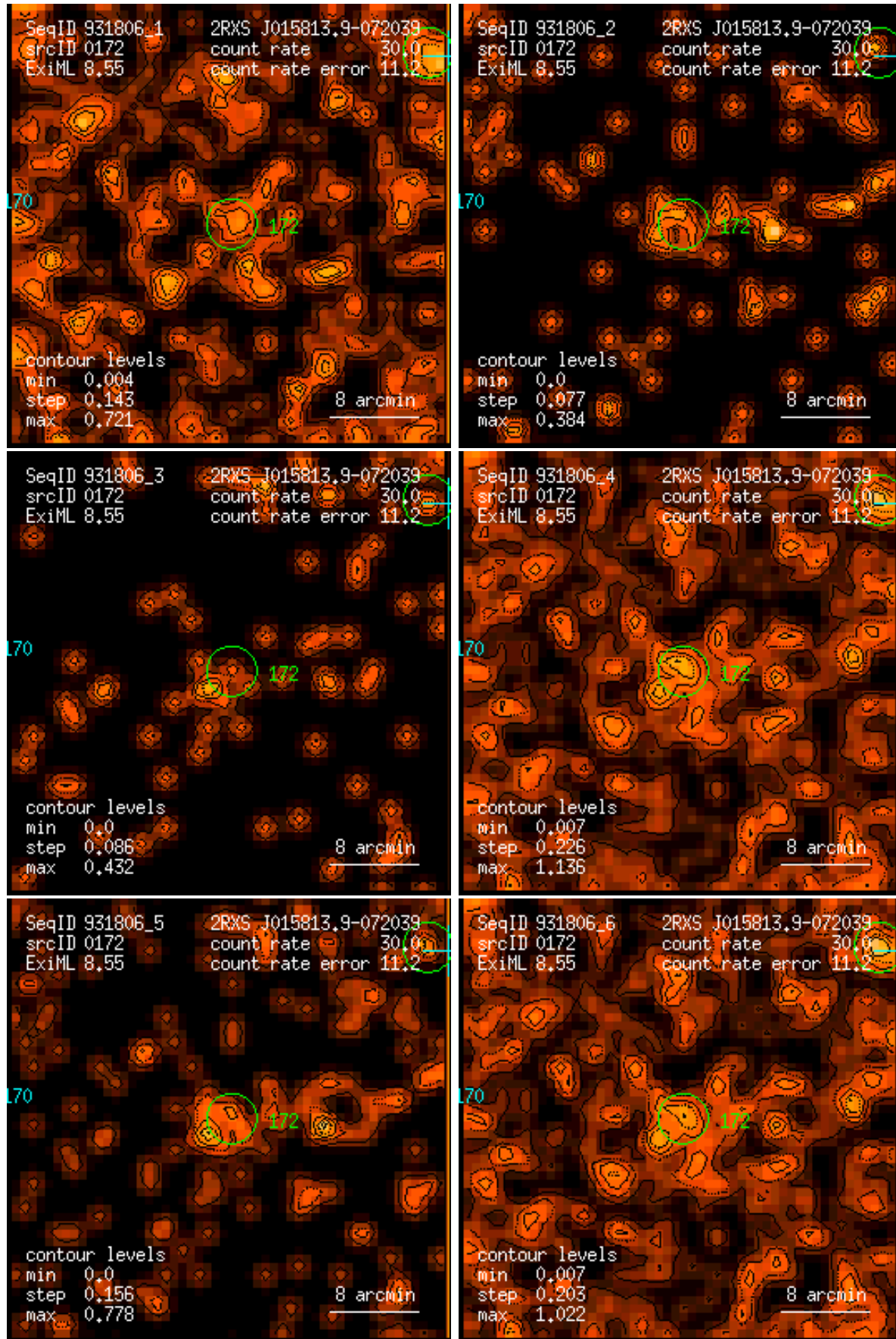
Figure 172: RASS 931806: detection 0172: band rate images, Gaussian filter: (1) PSPC channels 11 – 41, (2) 52 – 90, (3) 91 – 201, (4) 11 – 235, (5) 52 – 201, (6) 11 – 201. Broad band rates in counts/ks. Band rate contour levels in counts/ks/arcmin 2 .
