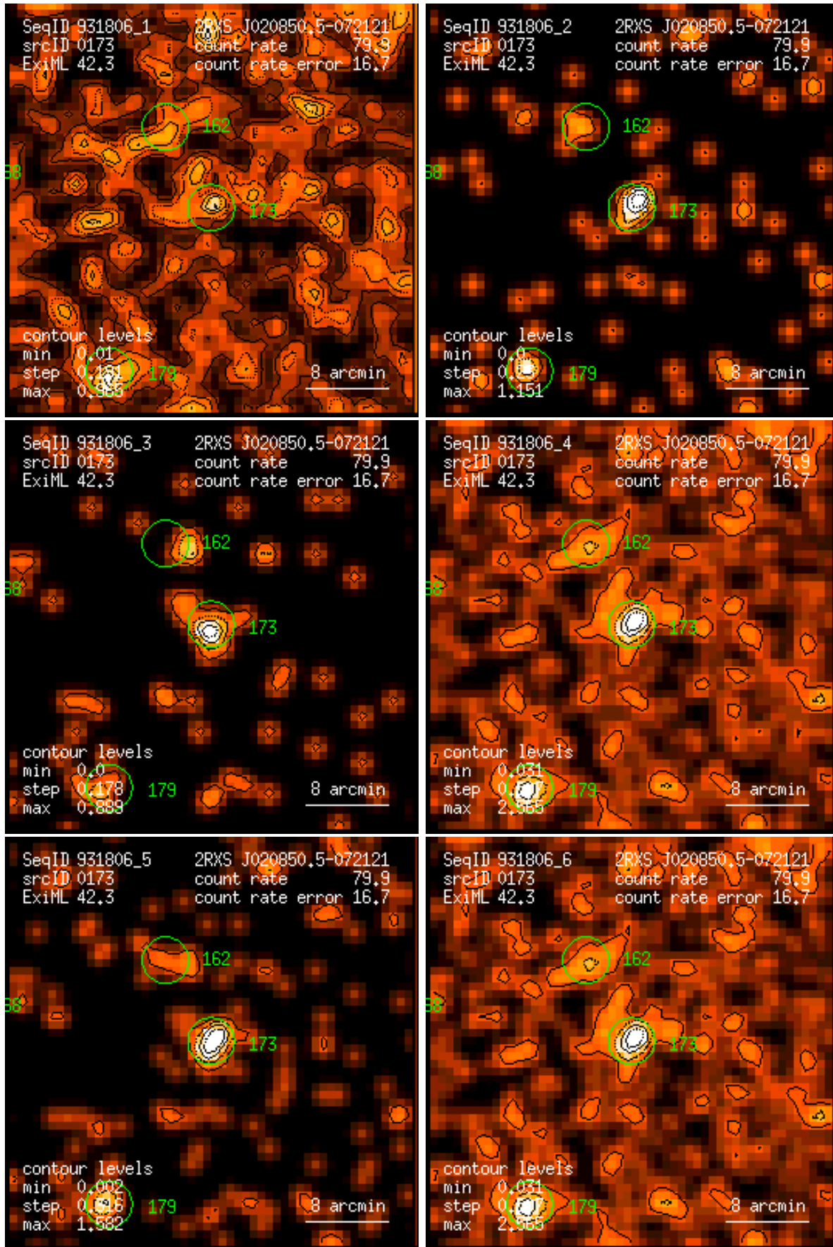
Figure 173: RASS 931806: detection 0173: band rate images, Gaussian filter: (1) PSPC channels 11 – 41, (2) 52 – 90, (3) 91 – 201, (4) 11 – 235, (5) 52 – 201, (6) 11 – 201. Broad band rates in counts/ks. Band rate contour levels in counts/ks/arcmin 2 .
