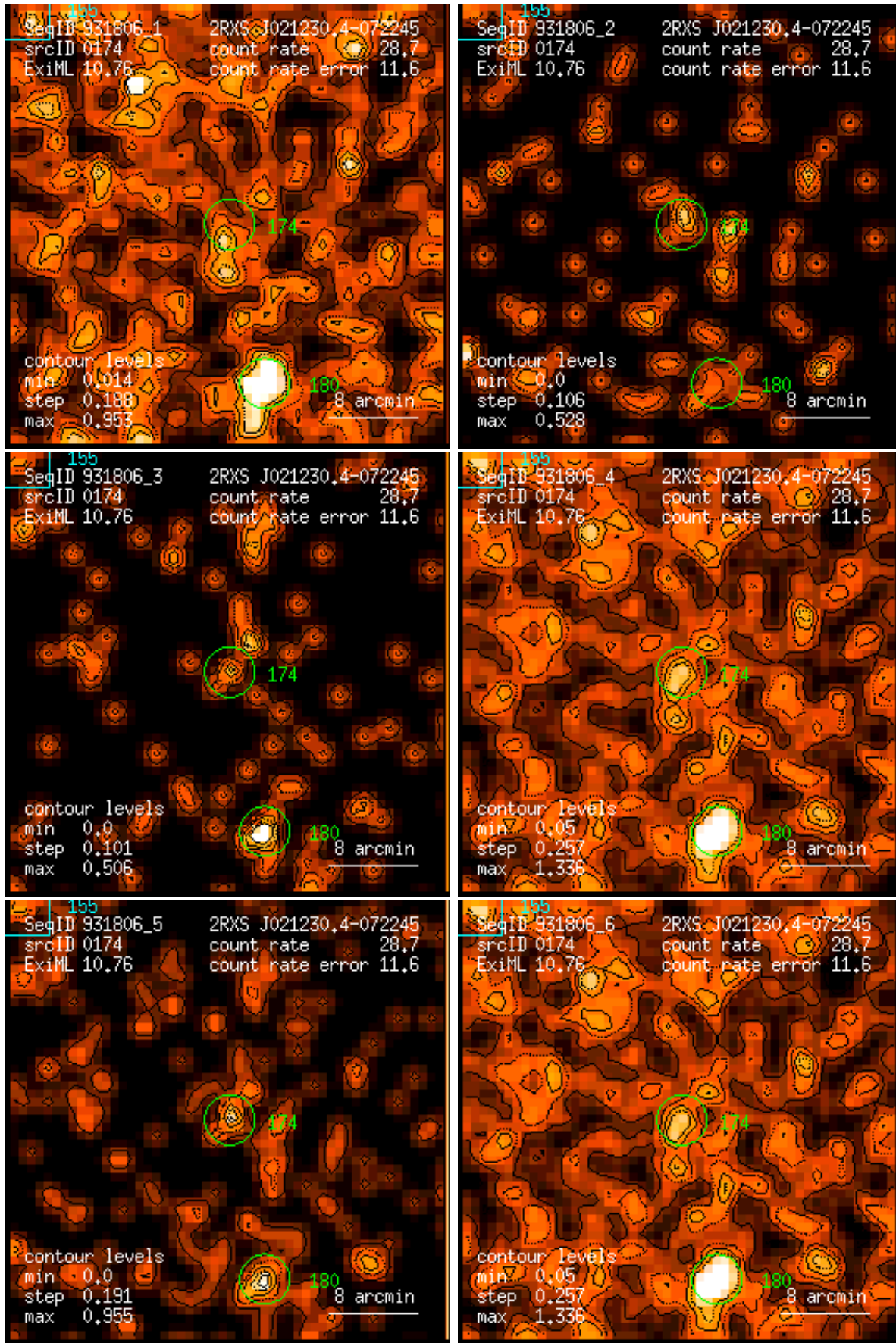
Figure 174: RASS 931806: detection 0174: band rate images, Gaussian filter: (1) PSPC channels 11 – 41, (2) 52 – 90, (3) 91 – 201, (4) 11 – 235, (5) 52 – 201, (6) 11 – 201. Broad band rates in counts/ks. Band rate contour levels in counts/ks/arcmin 2 .
