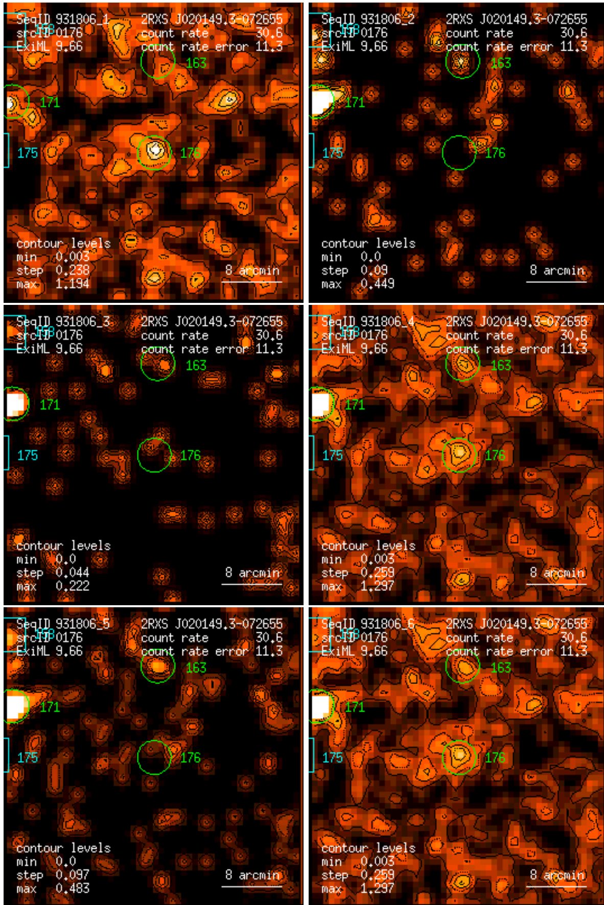
Figure 176: RASS 931806: detection 0176: band rate images, Gaussian filter: (1) PSPC channels 11 – 41, (2) 52 – 90, (3) 91 – 201, (4) 11 – 235, (5) 52 – 201, (6) 11 – 201. Broad band rates in counts/ks. Band rate contour levels in counts/ks/arcmin 2 .
