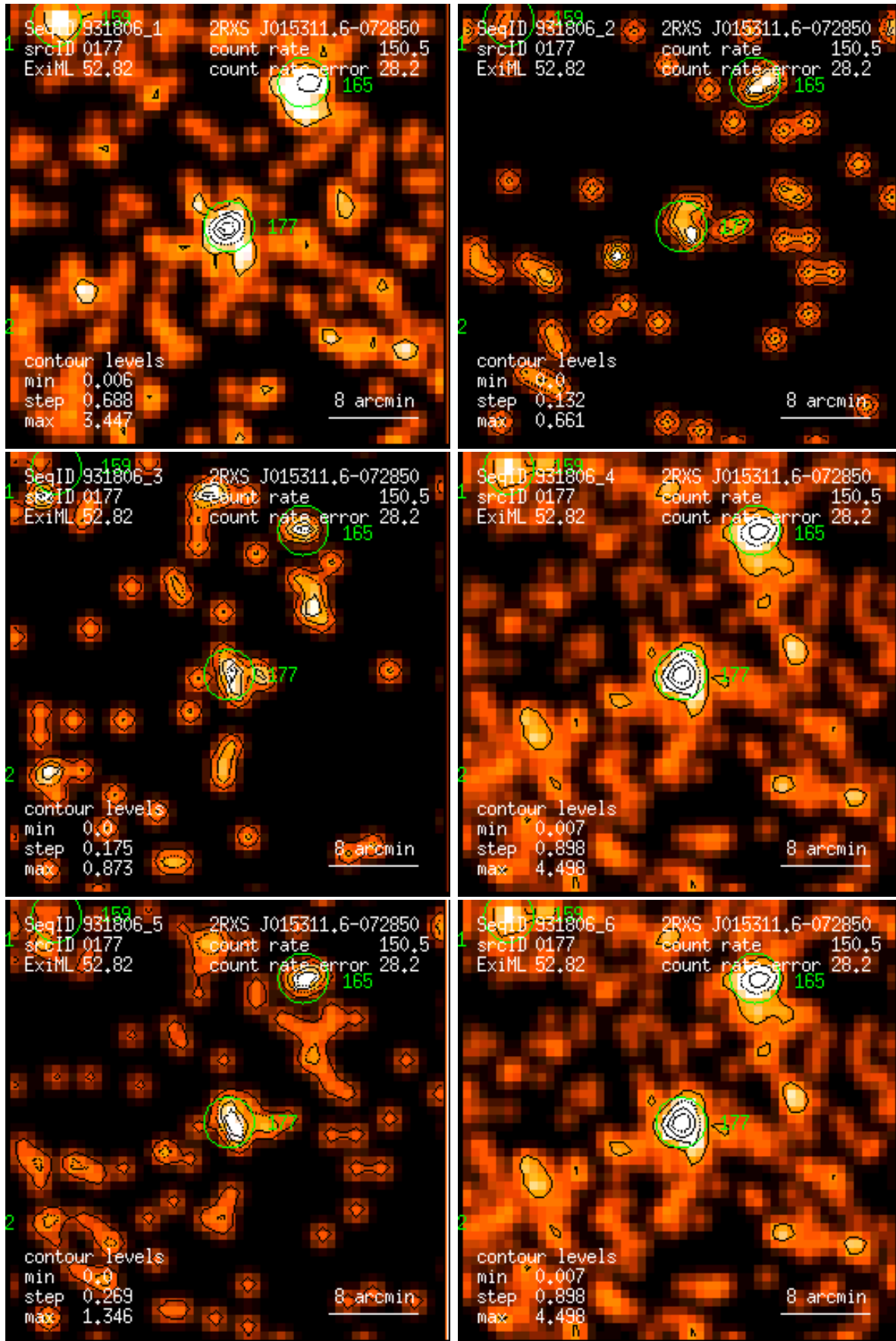
Figure 177: RASS 931806: detection 0177: band rate images, Gaussian filter: (1) PSPC channels 11 – 41, (2) 52 – 90, (3) 91 – 201, (4) 11 – 235, (5) 52 – 201, (6) 11 – 201. Broad band rates in counts/ks. Band rate contour levels in counts/ks/arcmin 2 .
