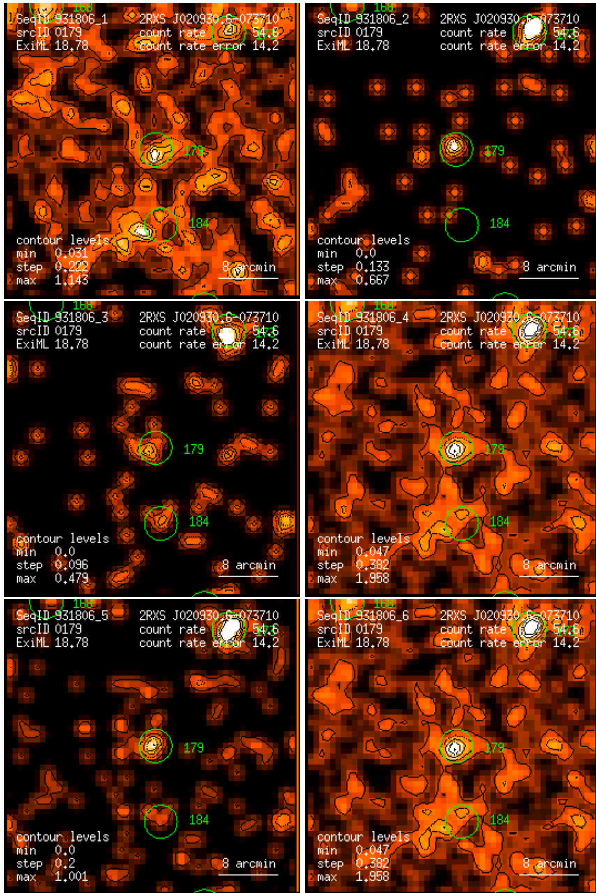
Figure 179: RASS 931806: detection 0179: band rate images, Gaussian filter: (1) PSPC channels 11 – 41, (2) 52 – 90, (3) 91 – 201, (4) 11 – 235, (5) 52 – 201, (6) 11 – 201. Broad band rates in counts/ks. Band rate contour levels in counts/ks/arcmin 2 .
