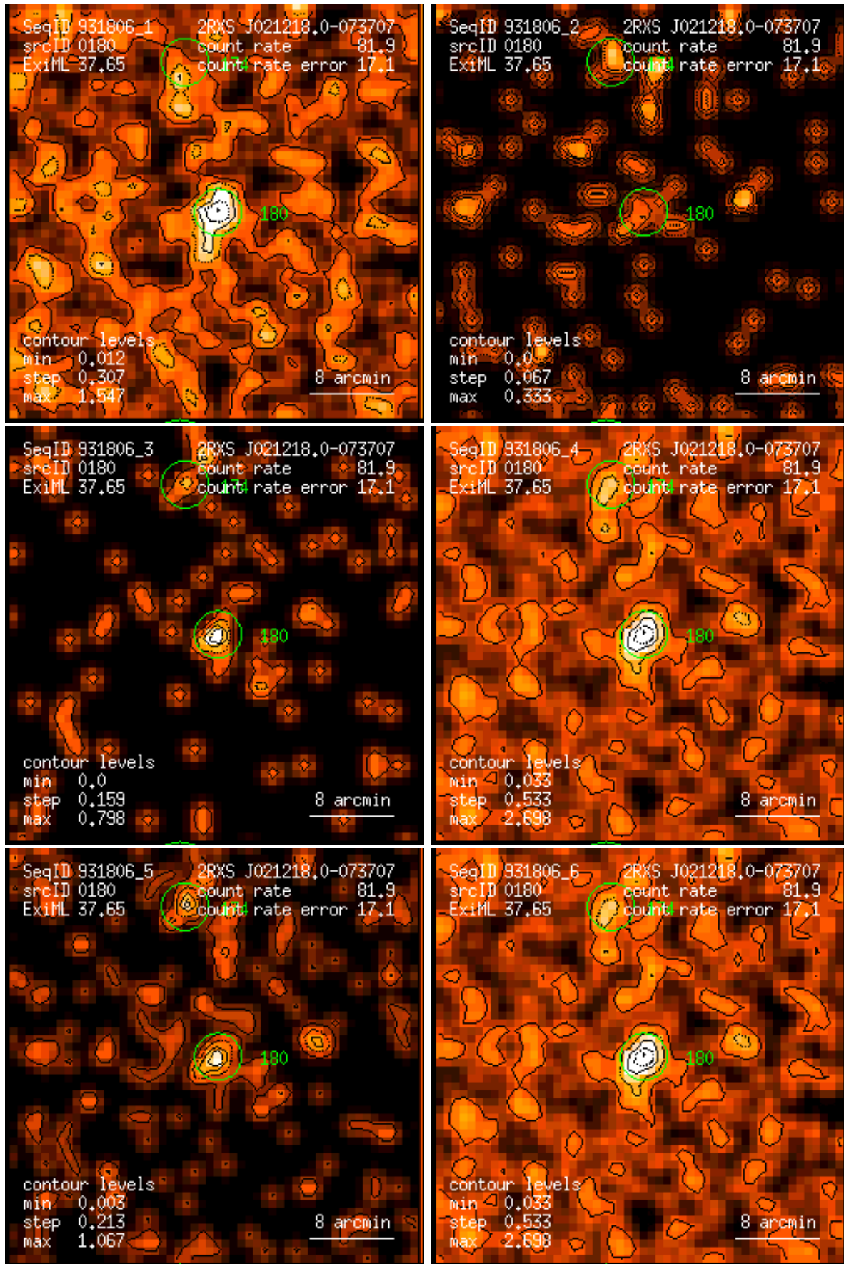
Figure 180: RASS 931806: detection 0180: band rate images, Gaussian filter: (1) PSPC channels 11 – 41, (2) 52 – 90, (3) 91 – 201, (4) 11 – 235, (5) 52 – 201, (6) 11 – 201. Broad band rates in counts/ks. Band rate contour levels in counts/ks/arcmin 2 .
