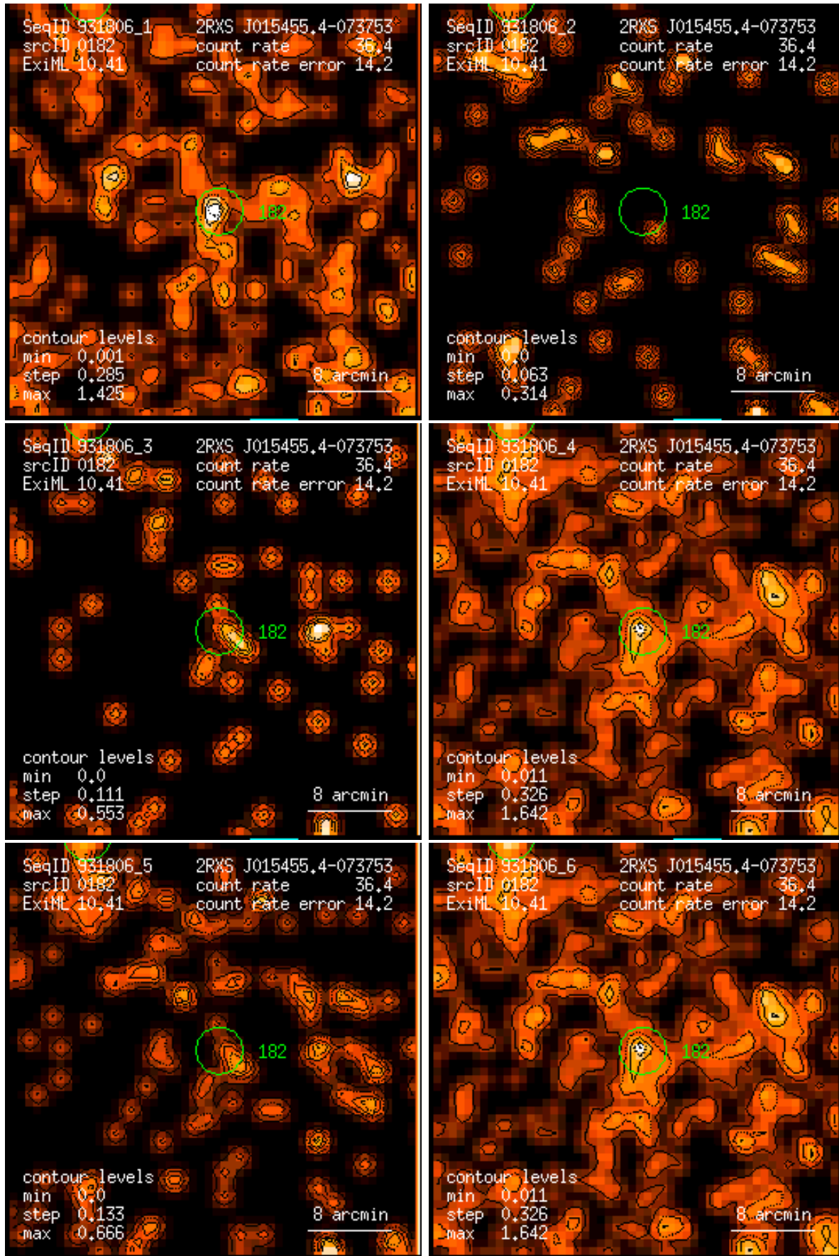
Figure 182: RASS 931806: detection 0182: band rate images, Gaussian filter: (1) PSPC channels 11 – 41, (2) 52 – 90, (3) 91 – 201, (4) 11 – 235, (5) 52 – 201, (6) 11 – 201. Broad band rates in counts/ks. Band rate contour levels in counts/ks/arcmin 2 .
