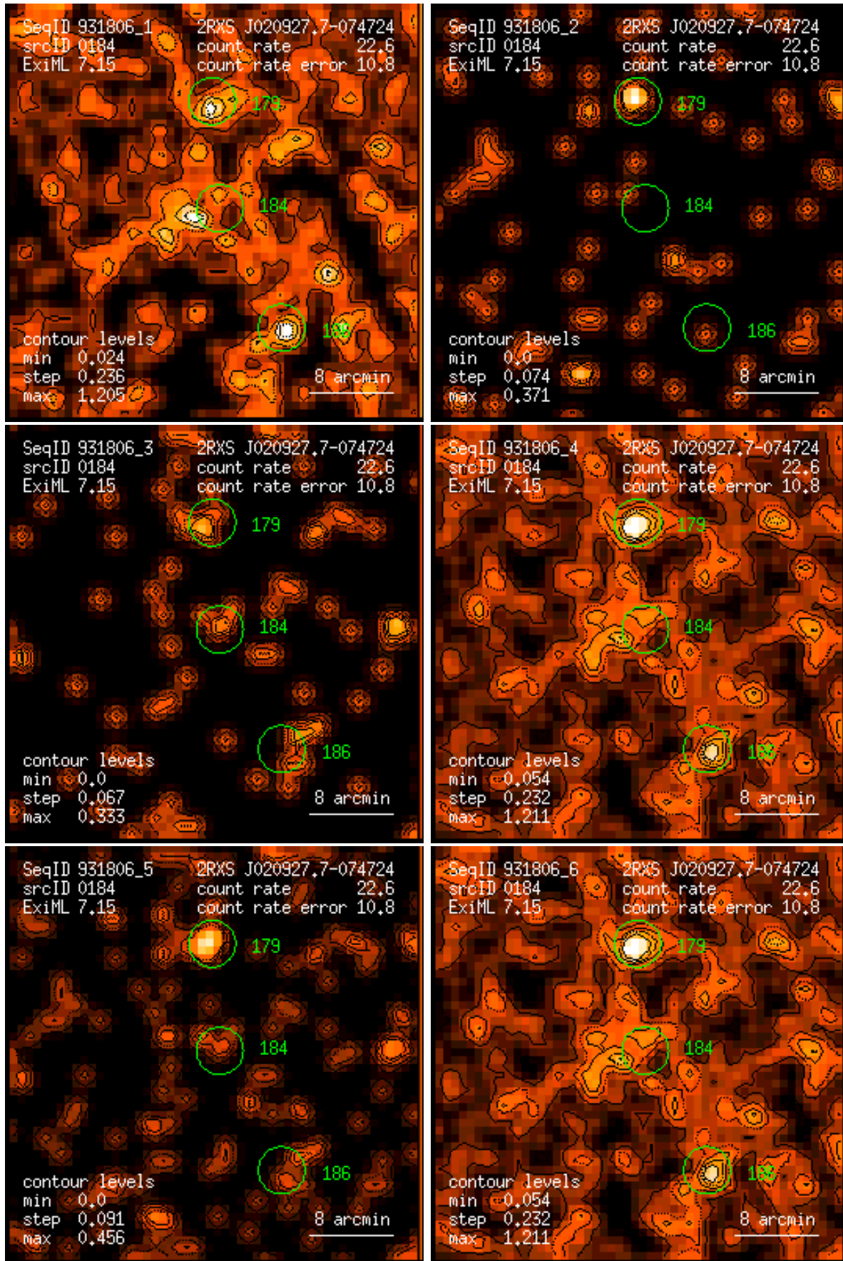
Figure 184: RASS 931806: detection 0184: band rate images, Gaussian filter: (1) PSPC channels 11 – 41, (2) 52 – 90, (3) 91 – 201, (4) 11 – 235, (5) 52 – 201, (6) 11 – 201. Broad band rates in counts/ks. Band rate contour levels in counts/ks/arcmin 2 .
