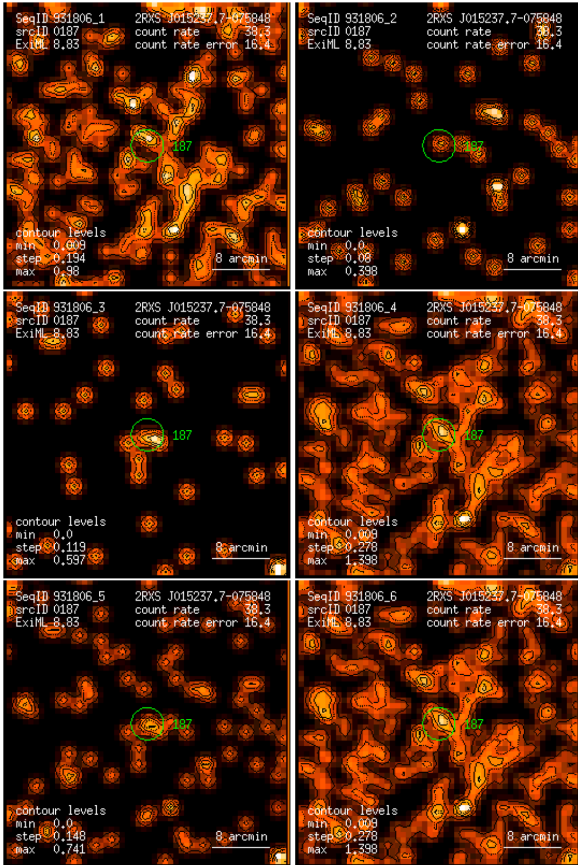
Figure 187: RASS 931806: detection 0187: band rate images, Gaussian filter: (1) PSPC channels 11 – 41, (2) 52 – 90, (3) 91 – 201, (4) 11 – 235, (5) 52 – 201, (6) 11 – 201. Broad band rates in counts/ks. Band rate contour levels in counts/ks/arcmin 2 .
