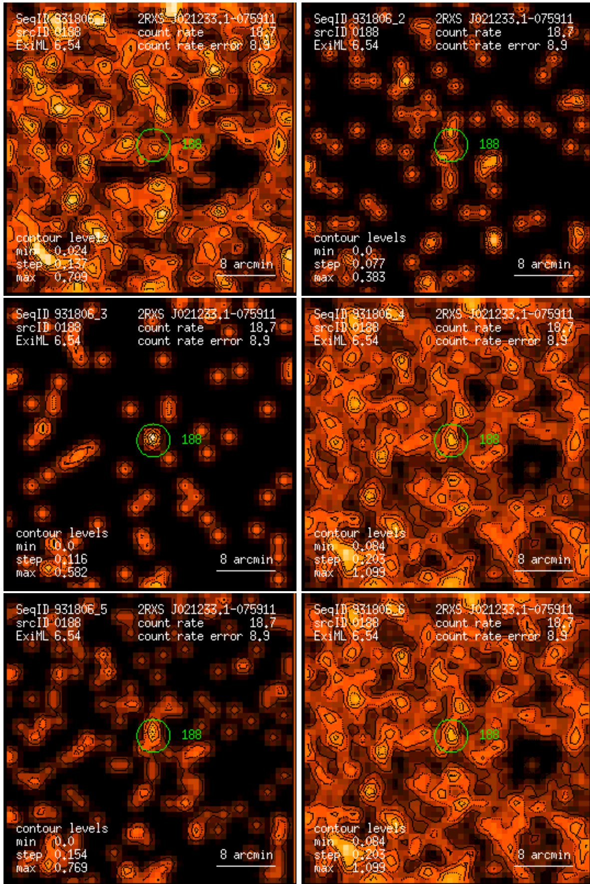
Figure 188: RASS 931806: detection 0188: band rate images, Gaussian filter: (1) PSPC channels 11 – 41, (2) 52 – 90, (3) 91 – 201, (4) 11 – 235, (5) 52 – 201, (6) 11 – 201. Broad band rates in counts/ks. Band rate contour levels in counts/ks/arcmin 2 .
