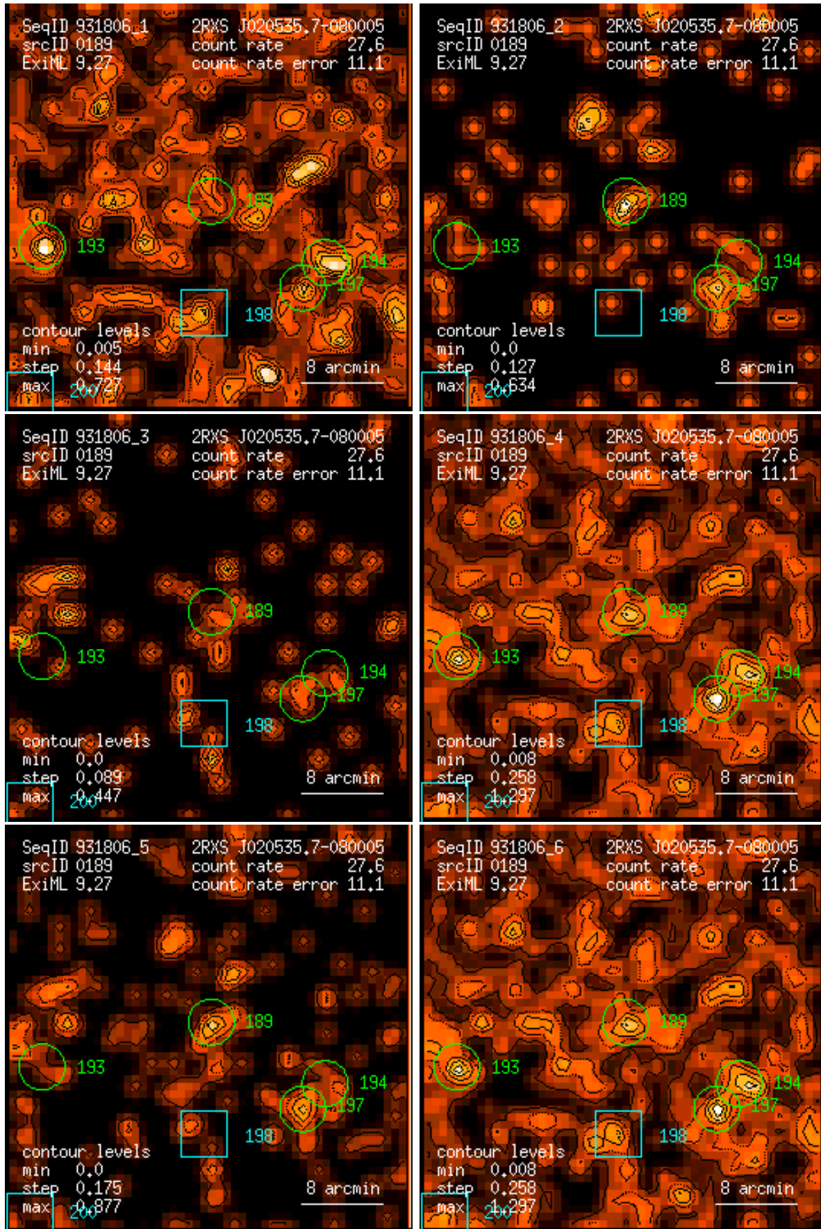
Figure 189: RASS 931806: detection 0189: band rate images, Gaussian filter: (1) PSPC channels 11 – 41, (2) 52 – 90, (3) 91 – 201, (4) 11 – 235, (5) 52 – 201, (6) 11 – 201. Broad band rates in counts/ks. Band rate contour levels in counts/ks/arcmin 2 .
