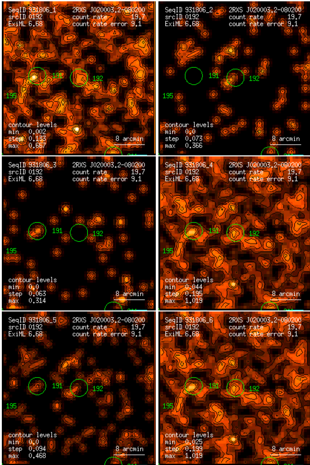
Figure 192: RASS 931806: detection 0192: band rate images, Gaussian filter: (1) PSPC channels 11 – 41, (2) 52 – 90, (3) 91 – 201, (4) 11 – 235, (5) 52 – 201, (6) 11 – 201. Broad band rates in counts/ks. Band rate contour levels in counts/ks/arcmin 2 .
