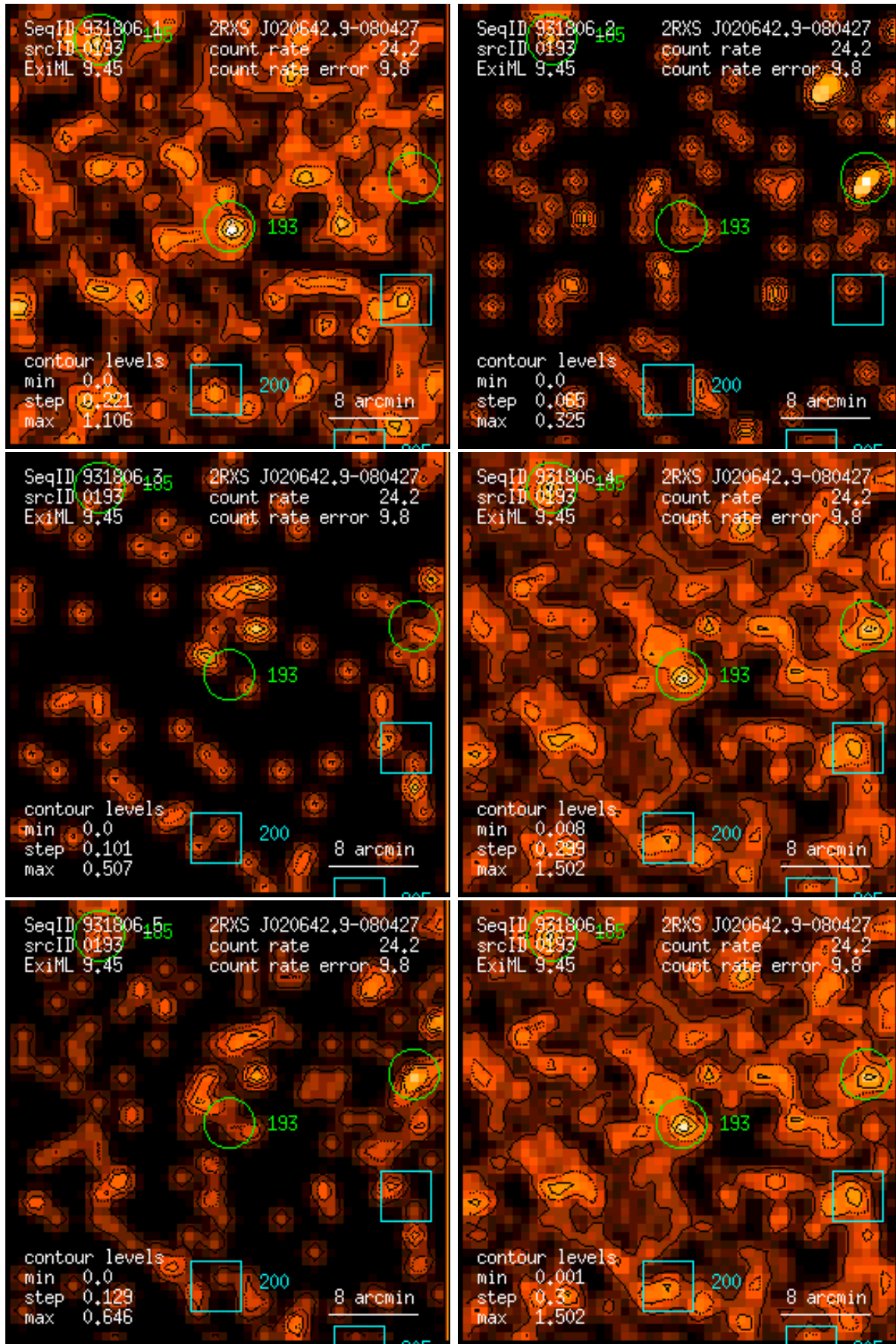
Figure 193: RASS 931806: detection 0193: band rate images, Gaussian filter: (1) PSPC channels 11 – 41, (2) 52 – 90, (3) 91 – 201, (4) 11 – 235, (5) 52 – 201, (6) 11 – 201. Broad band rates in counts/ks. Band rate contour levels in counts/ks/arcmin 2 .
