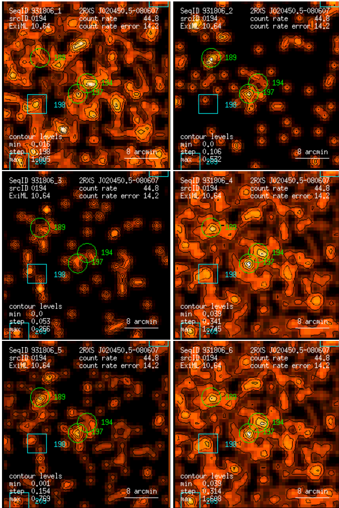
Figure 194: RASS 931806: detection 0194: band rate images, Gaussian filter: (1) PSPC channels 11 – 41, (2) 52 – 90, (3) 91 – 201, (4) 11 – 235, (5) 52 – 201, (6) 11 – 201. Broad band rates in counts/ks. Band rate contour levels in counts/ks/arcmin 2 .
