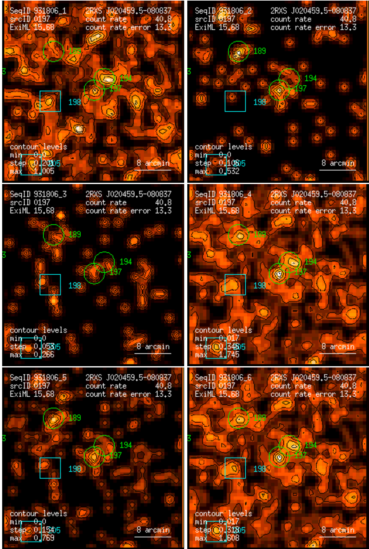
Figure 197: RASS 931806: detection 0197: band rate images, Gaussian filter: (1) PSPC channels 11 – 41, (2) 52 – 90, (3) 91 – 201, (4) 11 – 235, (5) 52 – 201, (6) 11 – 201. Broad band rates in counts/ks. Band rate contour levels in counts/ks/arcmin 2 .
