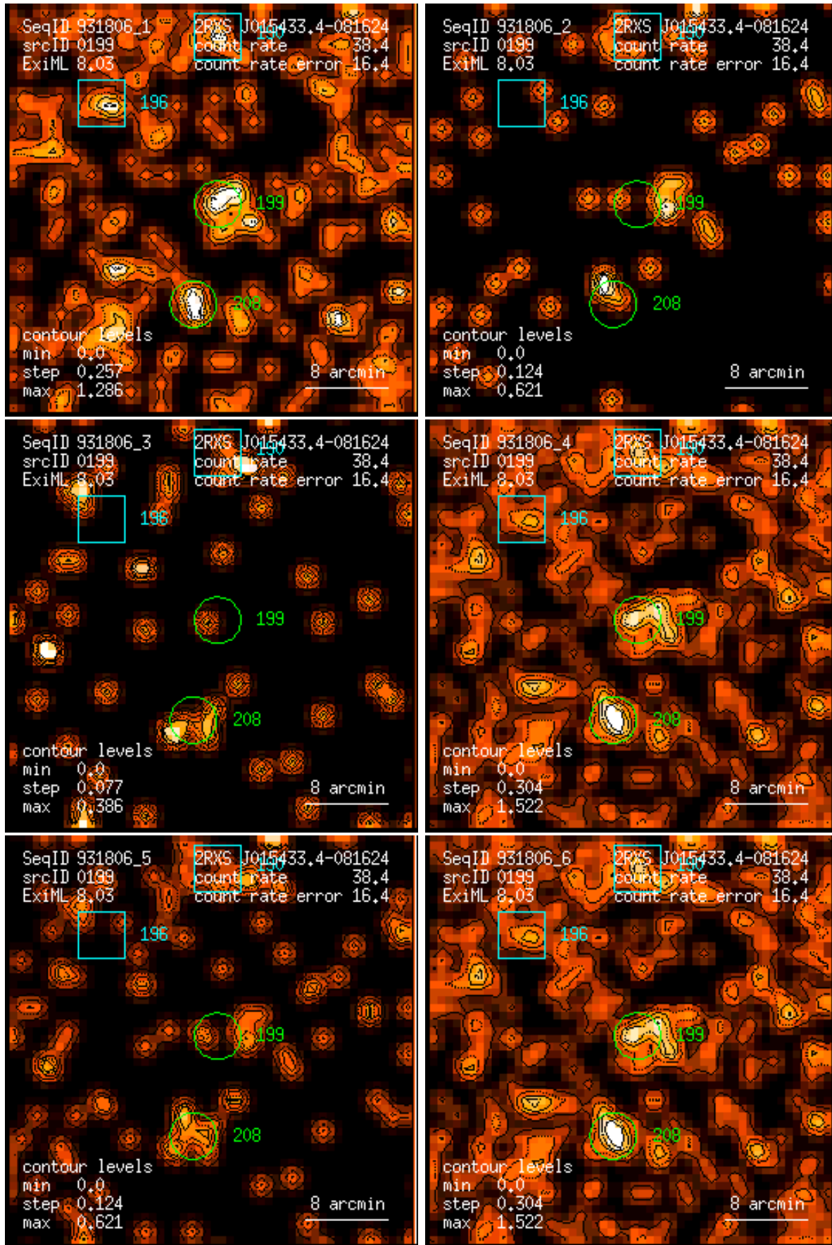
Figure 199: RASS 931806: detection 0199: band rate images, Gaussian filter: (1) PSPC channels 11 – 41, (2) 52 – 90, (3) 91 – 201, (4) 11 – 235, (5) 52 – 201, (6) 11 – 201. Broad band rates in counts/ks. Band rate contour levels in counts/ks/arcmin 2 .
