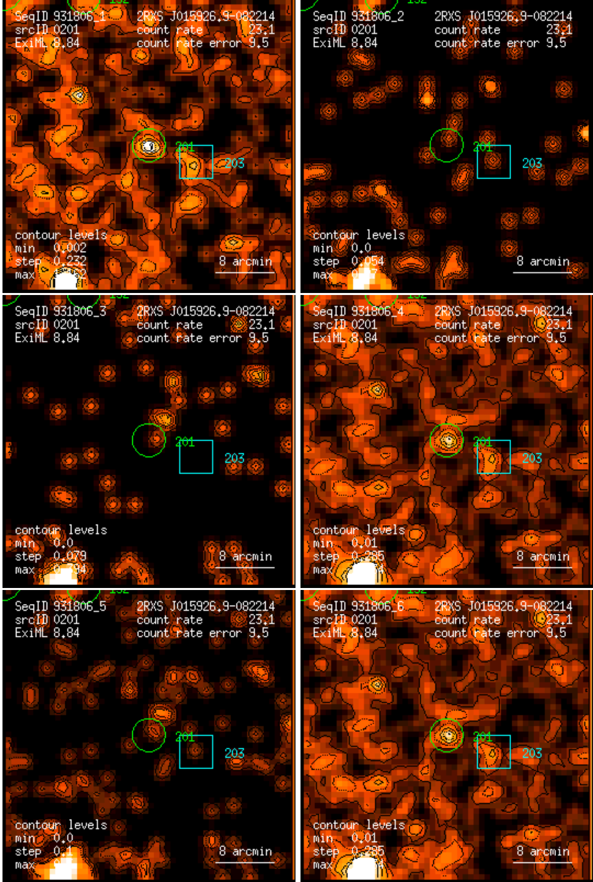
Figure 201: RASS 931806: detection 0201: band rate images, Gaussian filter: (1) PSPC channels 11 – 41, (2) 52 – 90, (3) 91 – 201, (4) 11 – 235, (5) 52 – 201, (6) 11 – 201. Broad band rates in counts/ks. Band rate contour levels in counts/ks/arcmin 2 .
