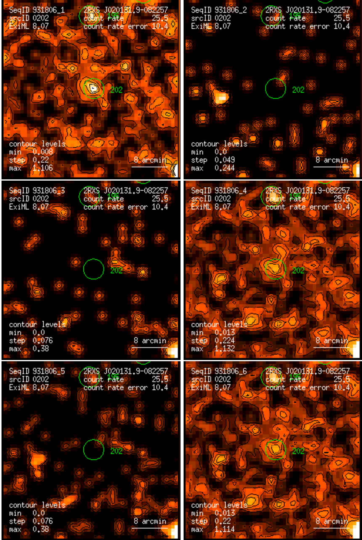
Figure 202: RASS 931806: detection 0202: band rate images, Gaussian filter: (1) PSPC channels 11 – 41, (2) 52 – 90, (3) 91 – 201, (4) 11 – 235, (5) 52 – 201, (6) 11 – 201. Broad band rates in counts/ks. Band rate contour levels in counts/ks/arcmin 2 .
