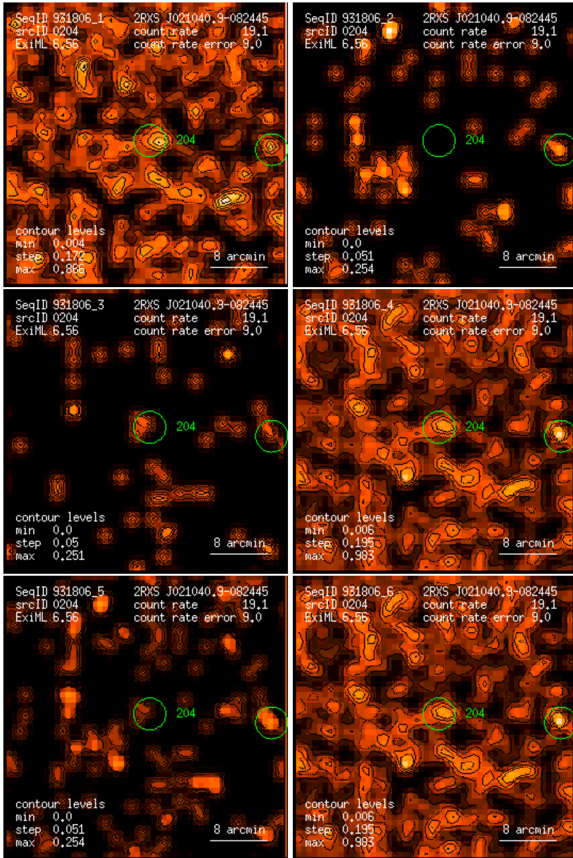
Figure 204: RASS 931806: detection 0204: band rate images, Gaussian filter: (1) PSPC channels 11 – 41, (2) 52 – 90, (3) 91 – 201, (4) 11 – 235, (5) 52 – 201, (6) 11 – 201. Broad band rates in counts/ks. Band rate contour levels in counts/ks/arcmin 2 .
